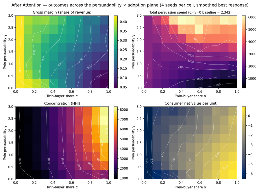
Figure 2: Outcomes across the persuadability × adoption plane. 16-point markup grid, M = 1,500 , 4 seeds per cell.
