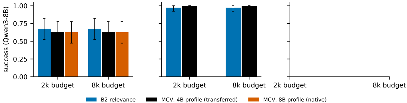
Facts (HotpotQA)
