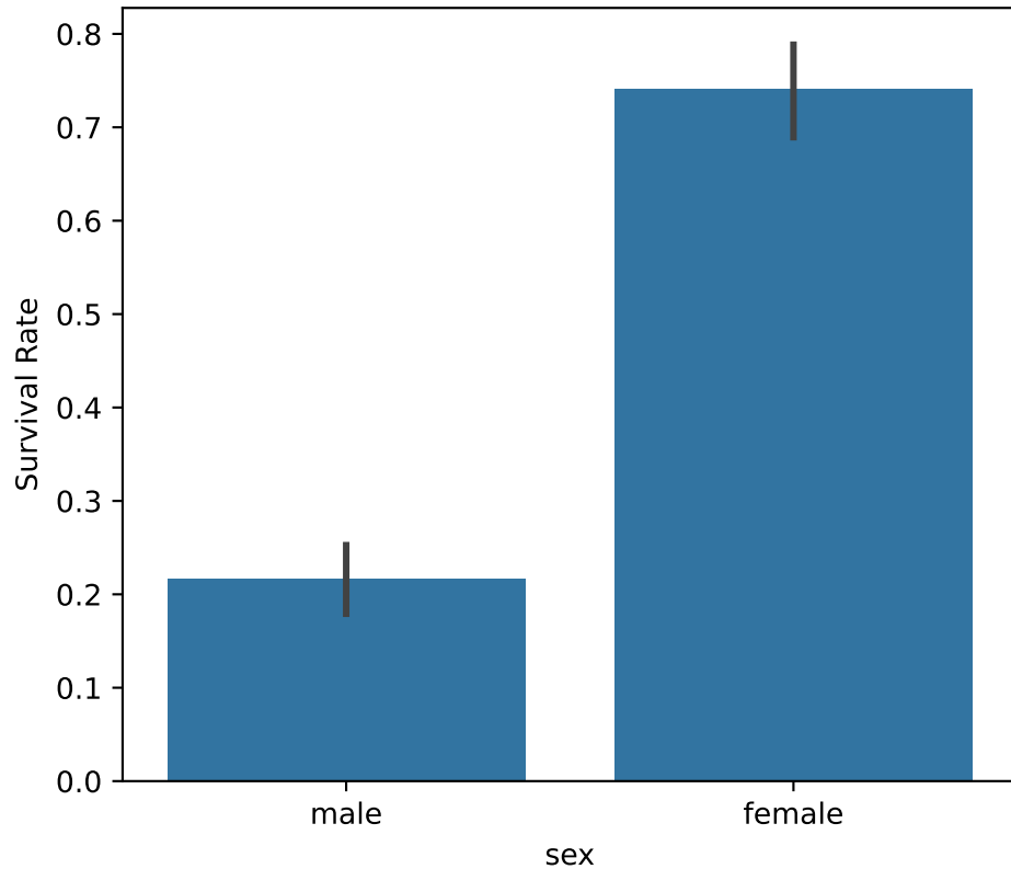
Survival Rate by Sex
