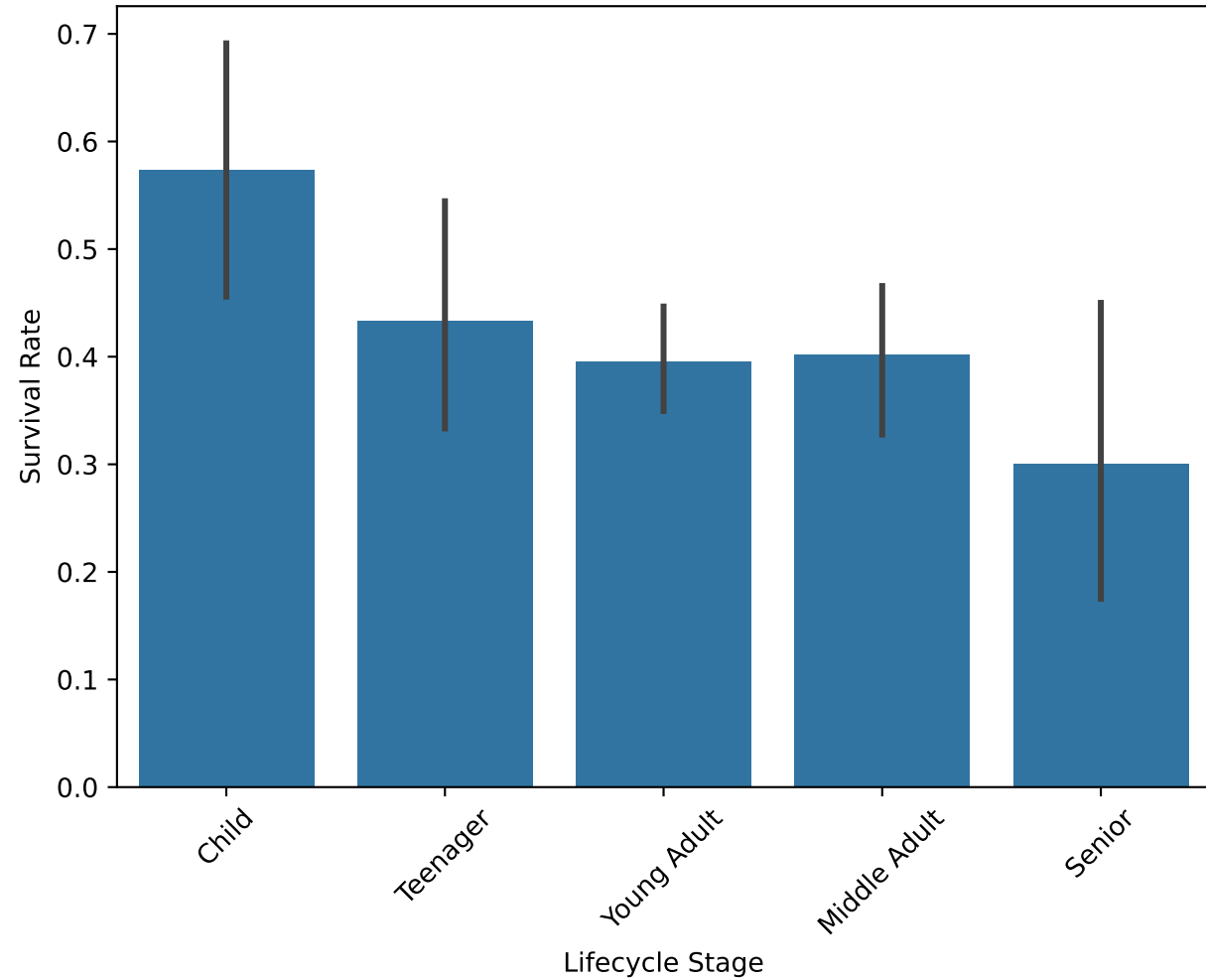
Survival Rate by Lifecycle
