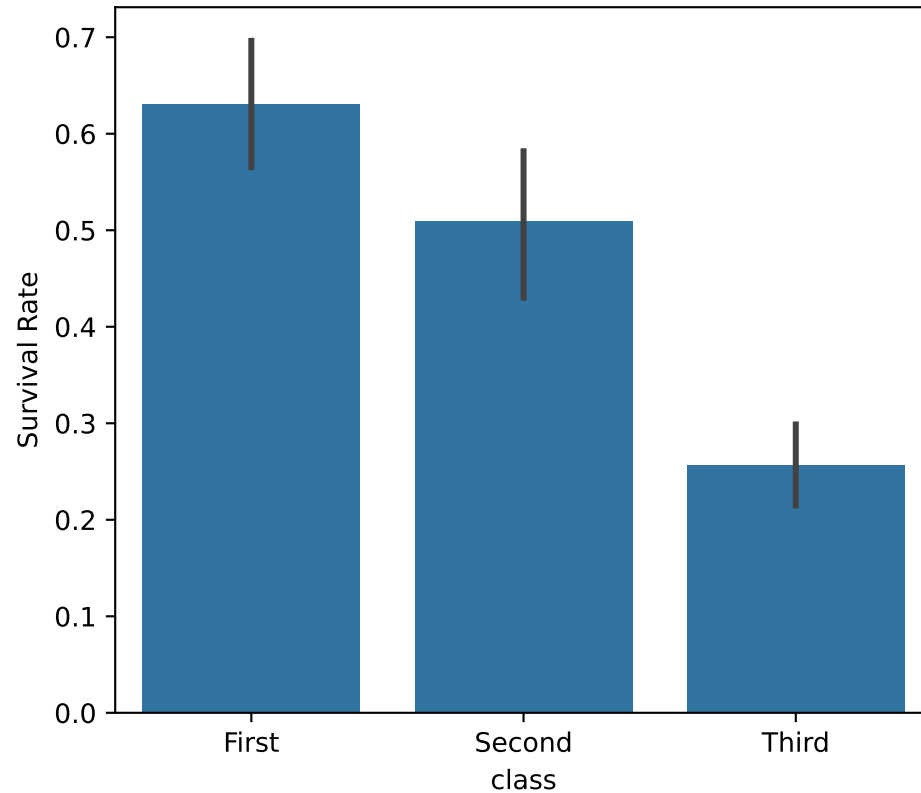
Survival Rate by Class
