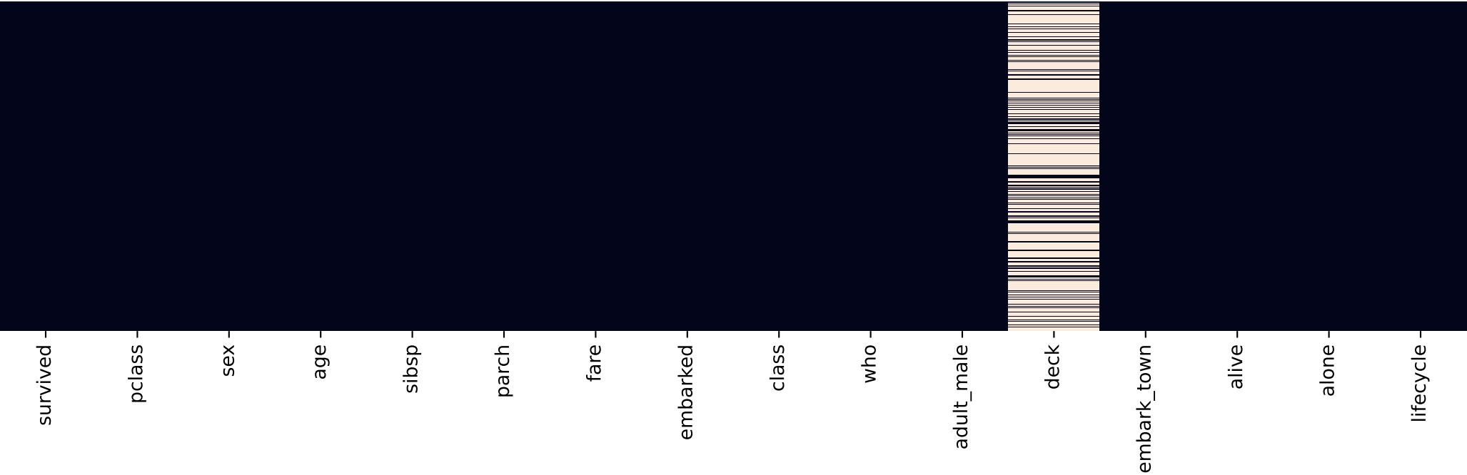
Missing-Value Heatmap
