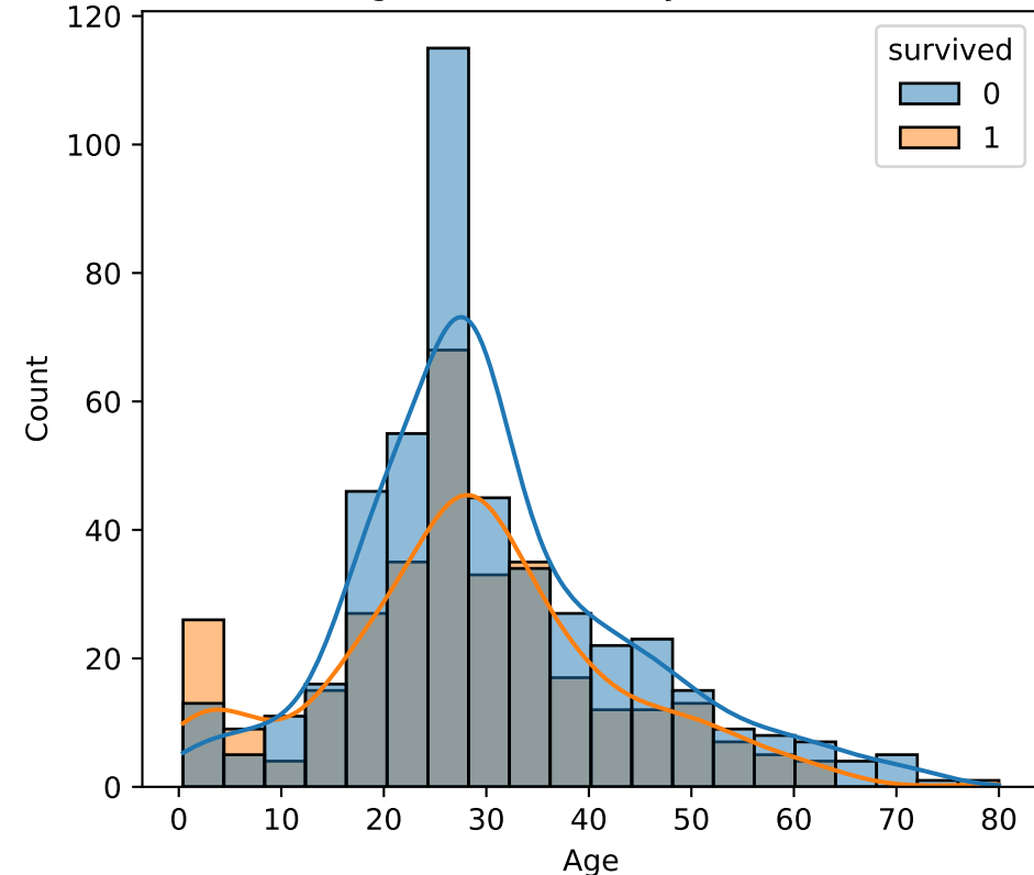
Age Distribution by Survival
