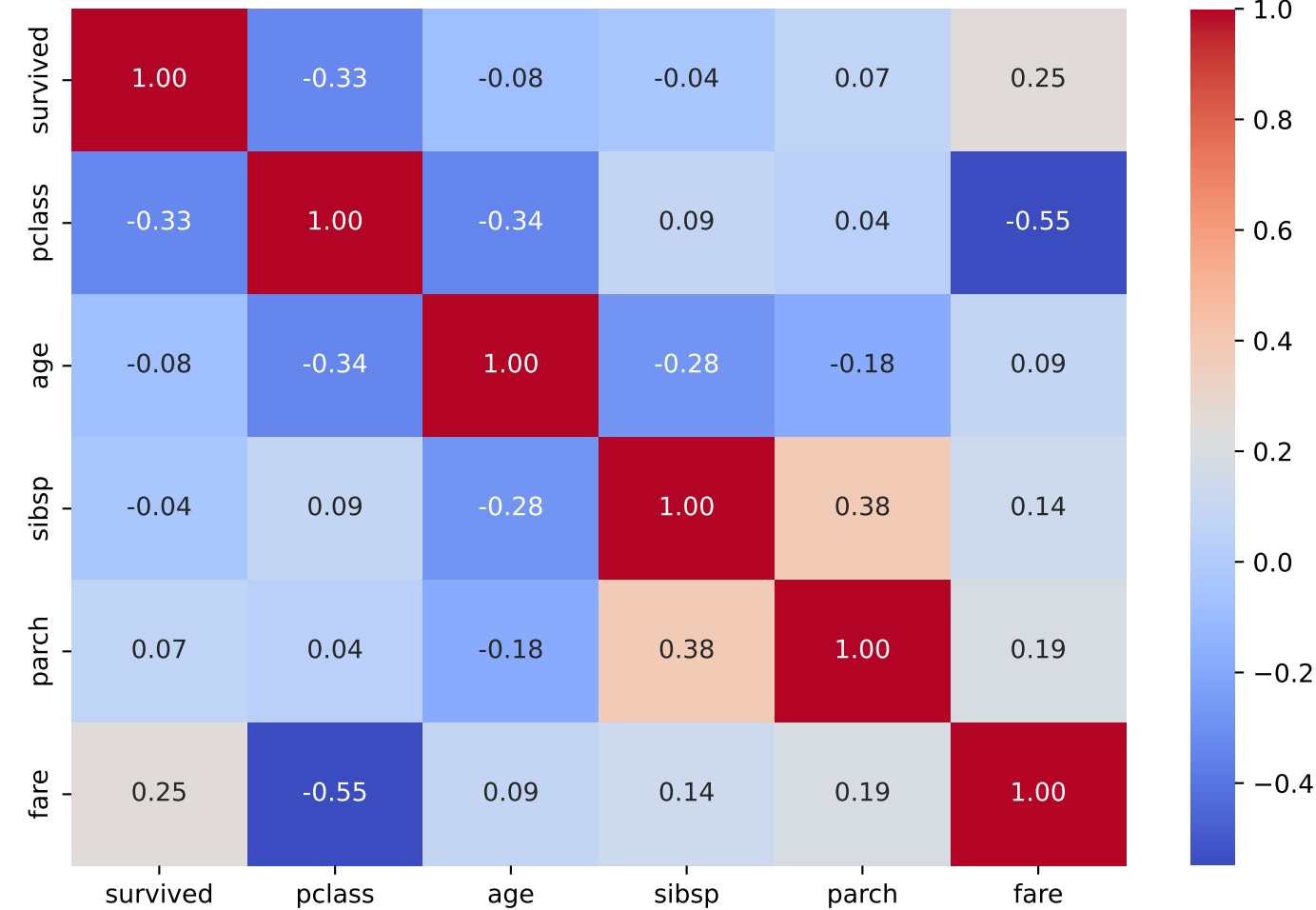
Correlation Heatmap
