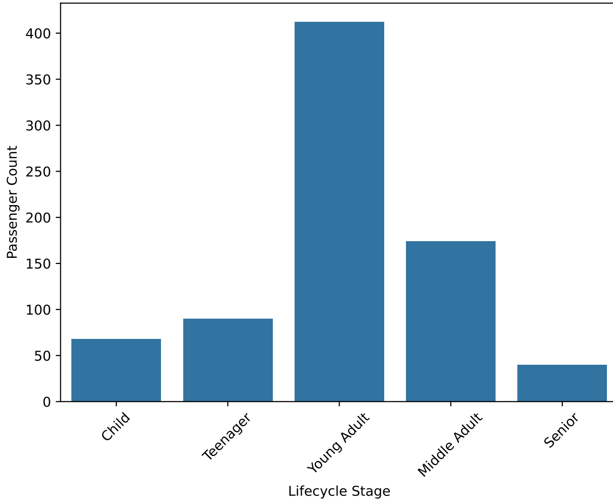
Passenger Count by Lifecycle
