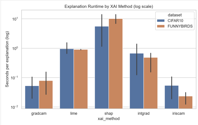
Fig. 3: Log-scale explanation runtime per sample. IRIS-CAM and Grad-CAM execute orders of magnitude faster than SHAP and Integrated Gradients.
