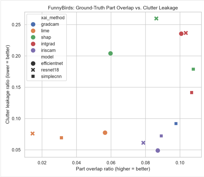
Fig. 2: Ground-Truth Part Overlap vs. Background Clutter Leakage on FunnyBirds. IRIS-CAM and Grad-CAM cluster in the ideal low-leakage zone.
