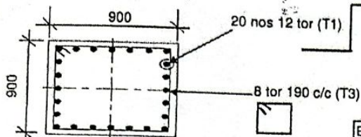
DETAIL OF PEDESTAL
