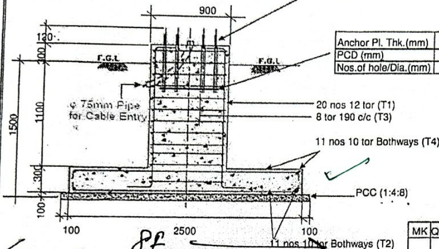
SECTIONAL ELEVATION
