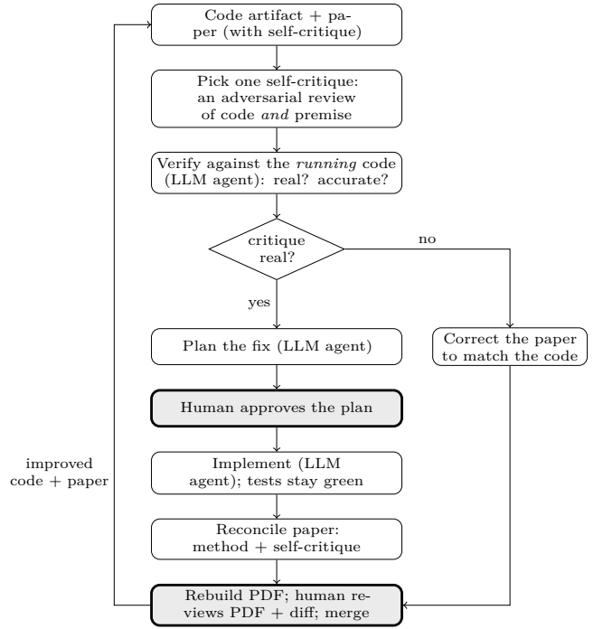
Figure 2: The reconcile-critique loop (§3.8): the paper’s self-critique drives revision of an executable artifact. Two human gates (shaded) bracket every change—plan approval and merge review. Verification and planning use one LLM agent; implementation a separate one. A pass that finds the critique unfounded corrects the paper instead of the code.
