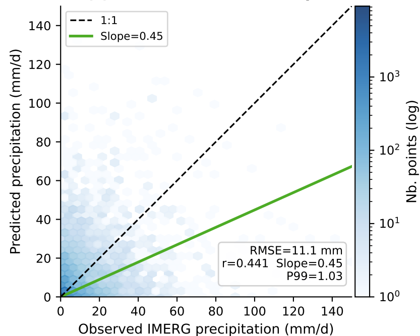
(c) UNet-CBAM — Base + QM
