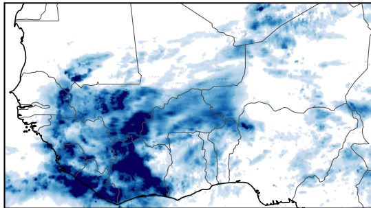
IMERG (observations)
