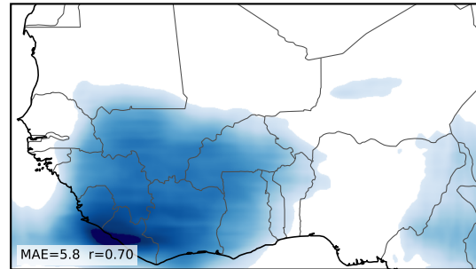
U-Net-CBAM
