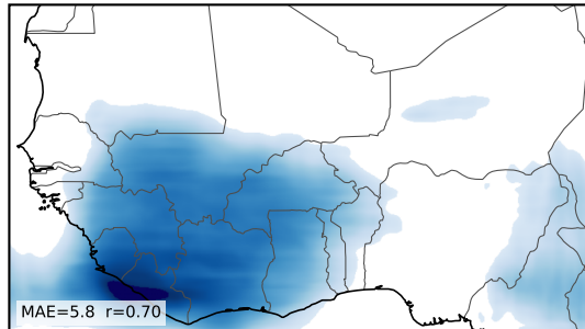
U-Net-CBAM
