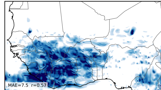
U-Net-CBAM cGAN
