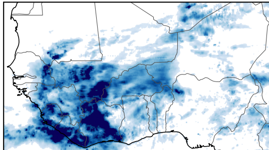
IMERG (observations)
