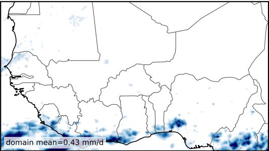
IMERG (observations)
