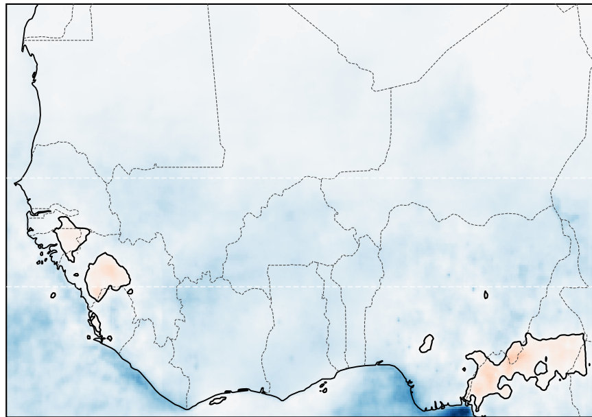
(a) Bias UNet-CBAM base (Predicted – Observed)
