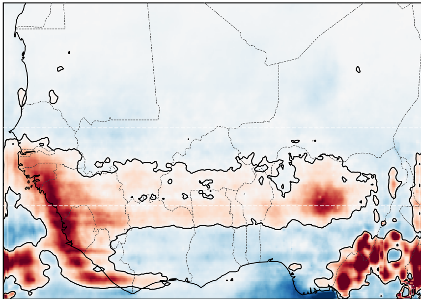
(b) Bias UNet-CBAM cGAN (Predicted – Observed)
