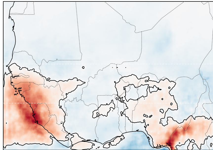
(c) Bias UNet-CBAM + QM (Predicted – Observed)
