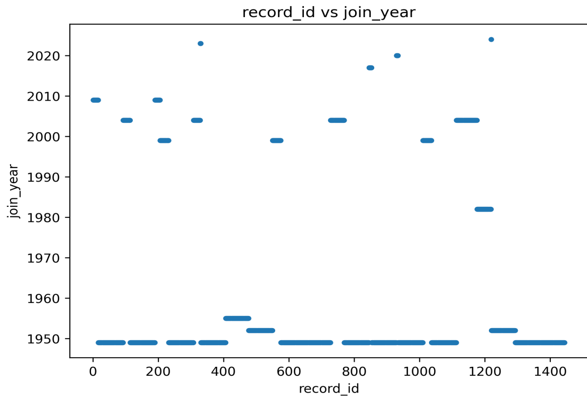
Scatter relationship between record_id and join_year.
