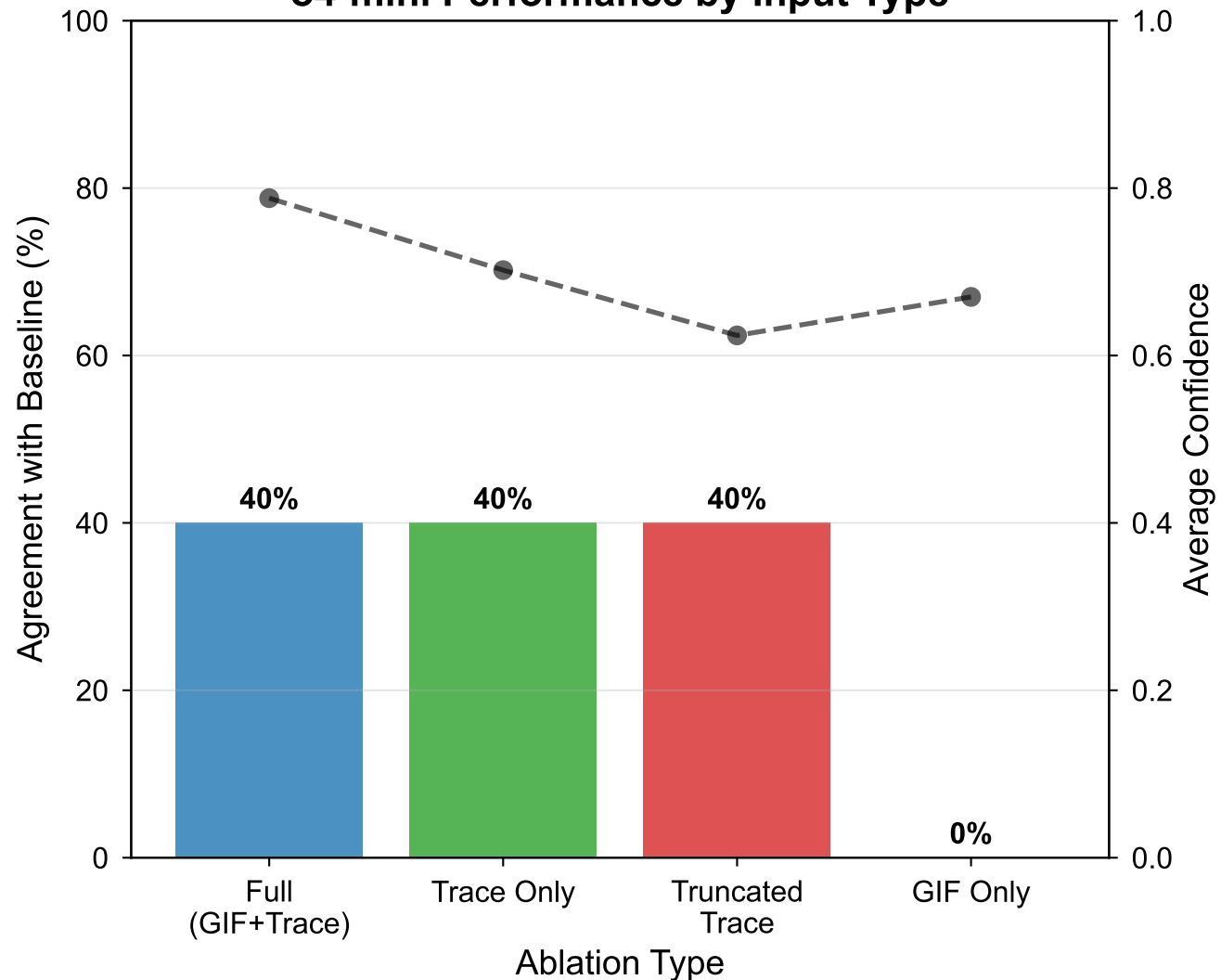
o4-mini Performance by Input Type
