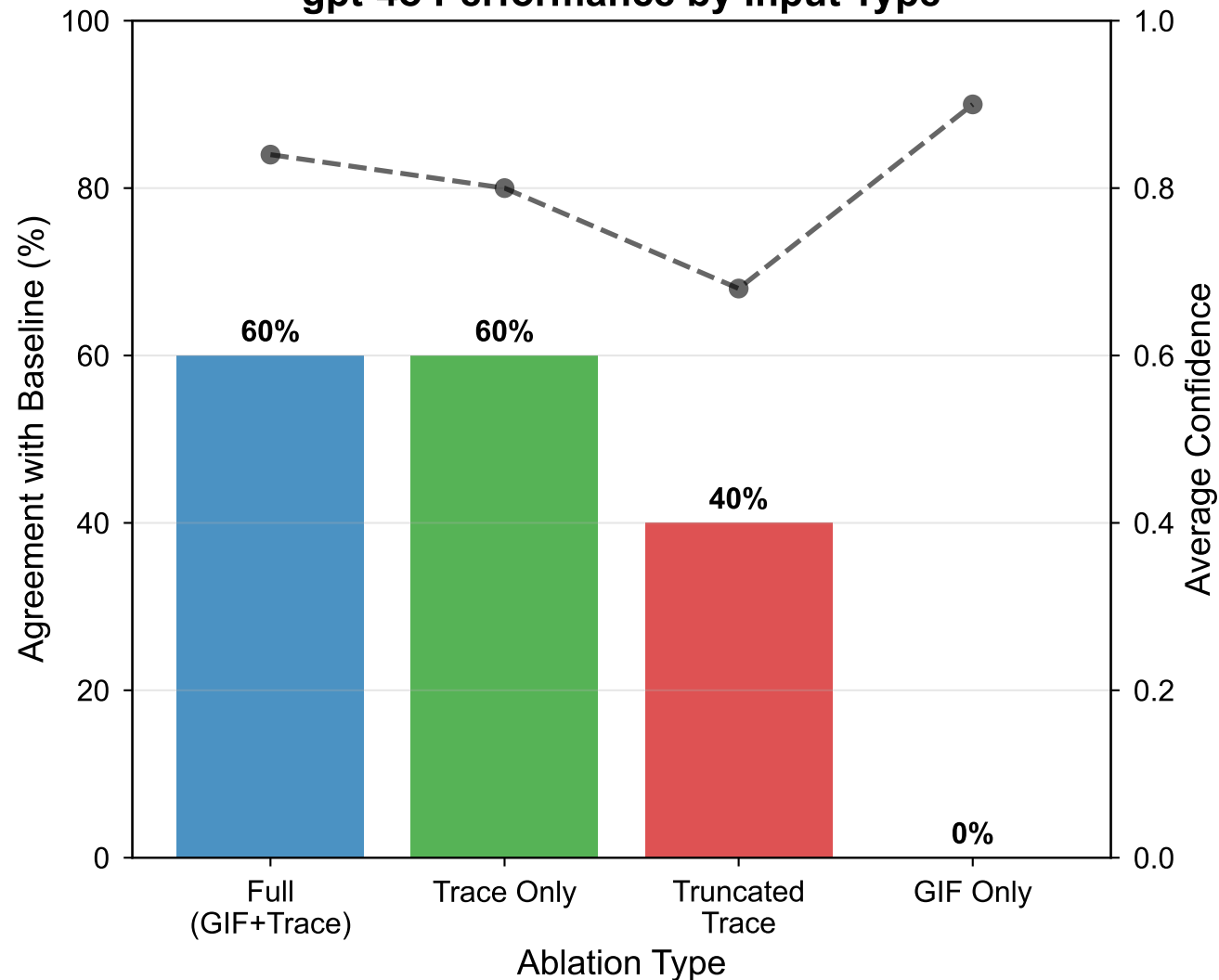
gpt-4o Performance by Input Type
