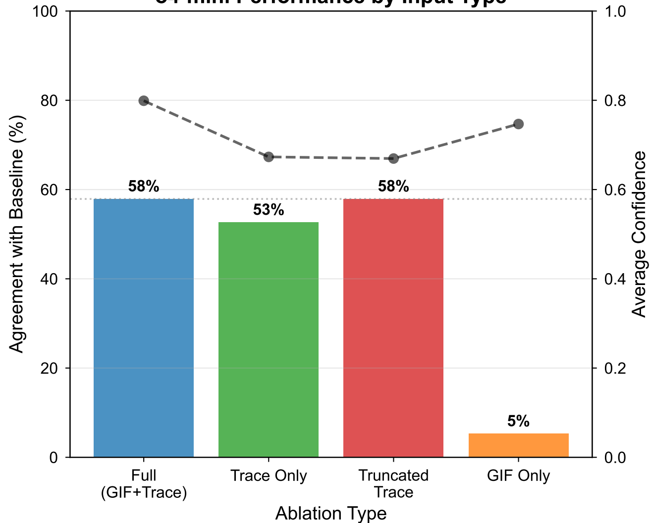
o4-mini Performance by Input Type
