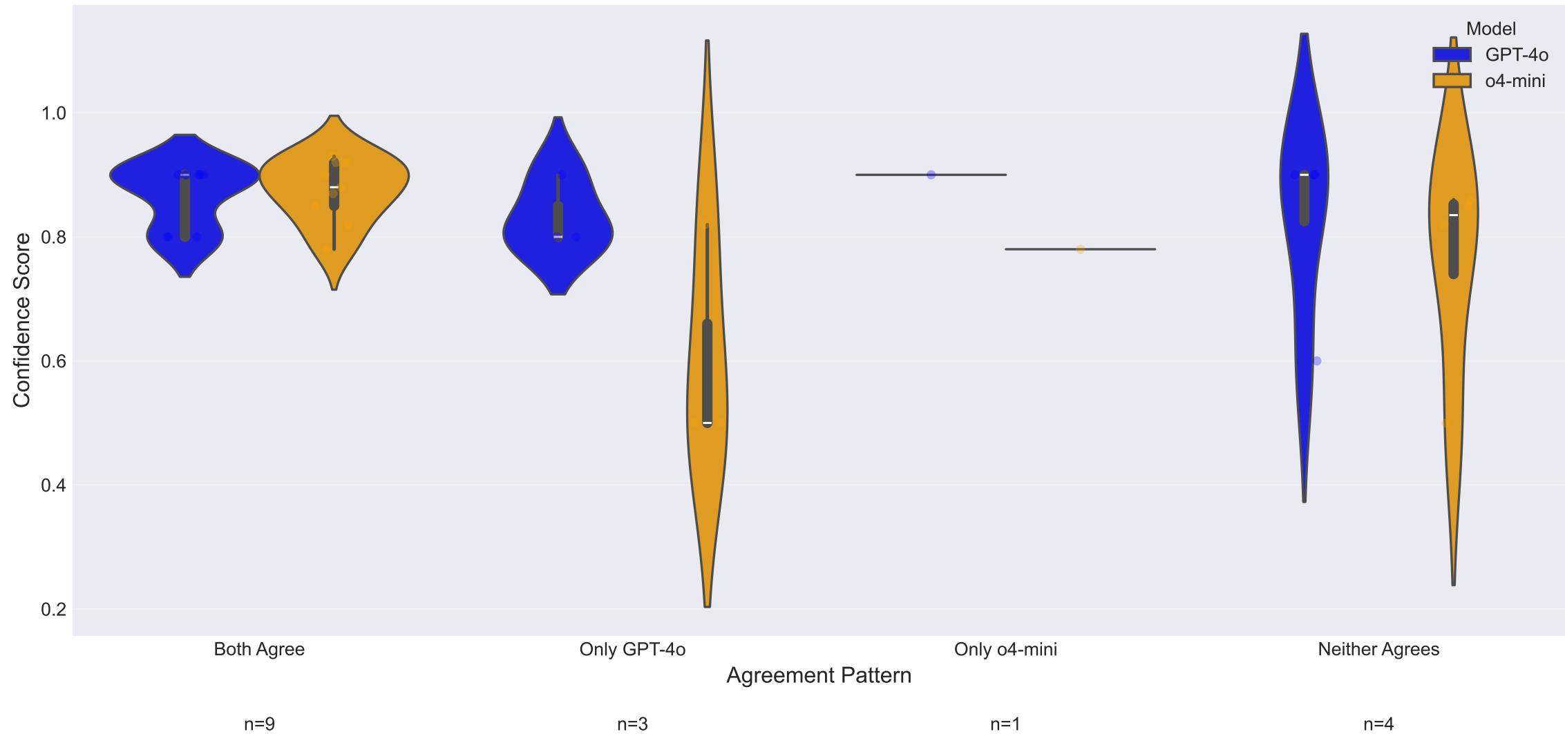
Model Confidence Distribution by Agreement with Baseline
