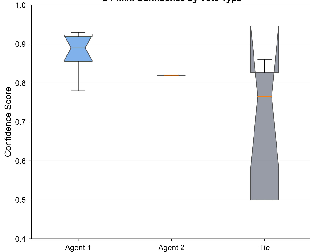
O4-mini Confidence by Vote Type
