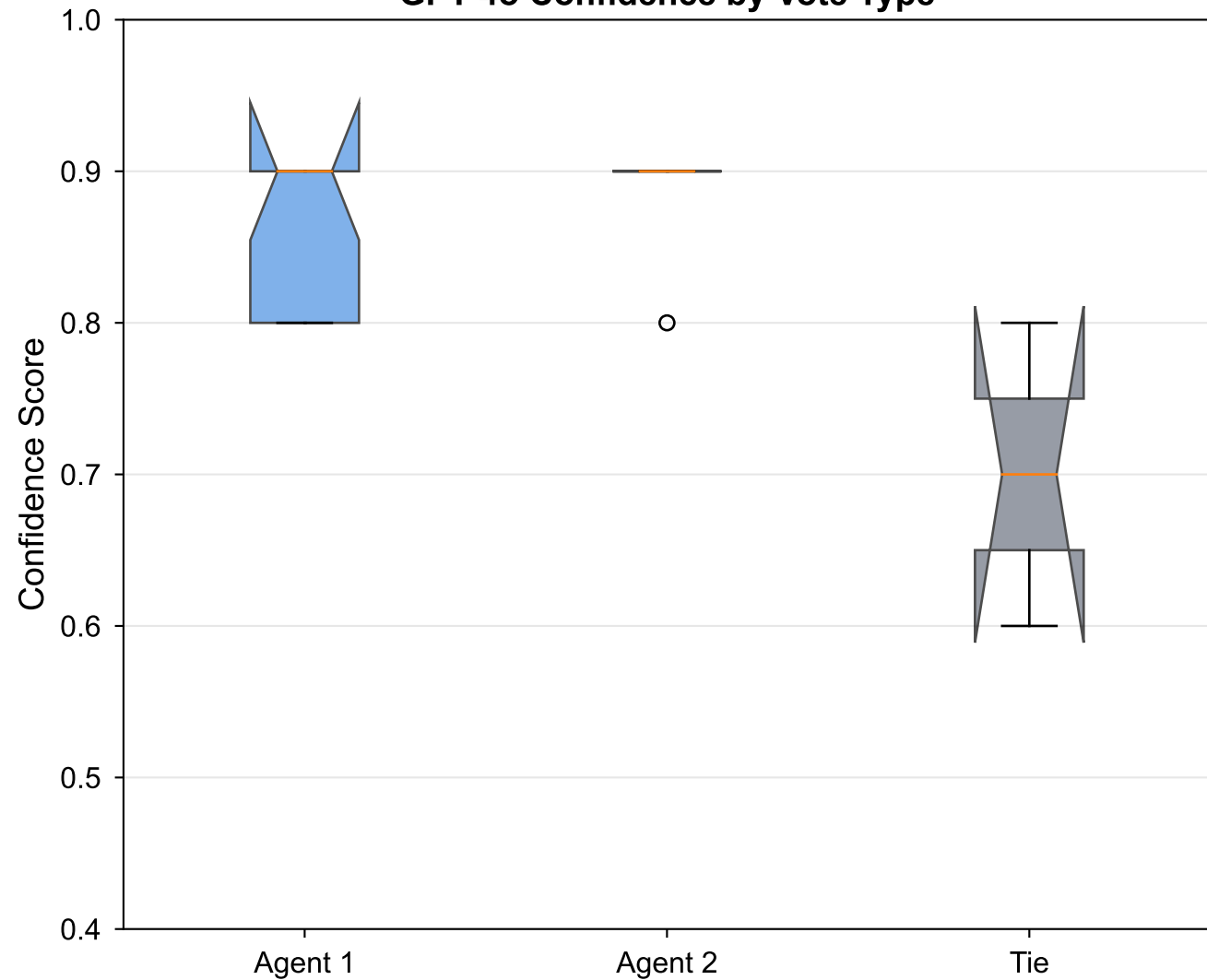
GPT-4o Confidence by Vote Type
