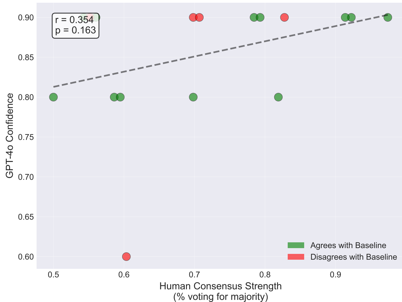
GPT-4o Confidence vs Human Consensus
