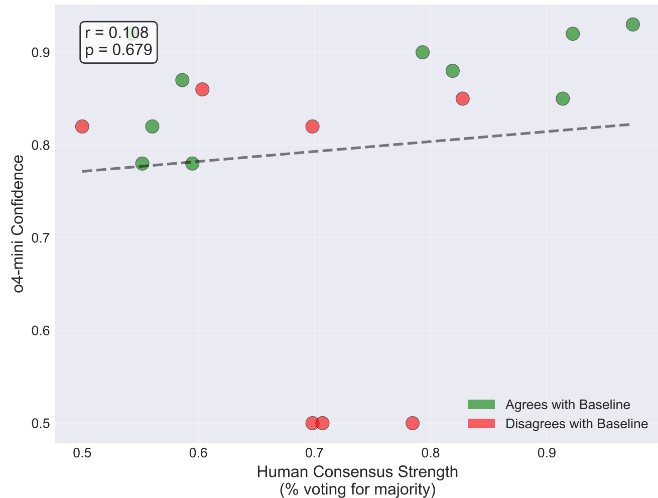
o4-mini Confidence vs Human Consensus
