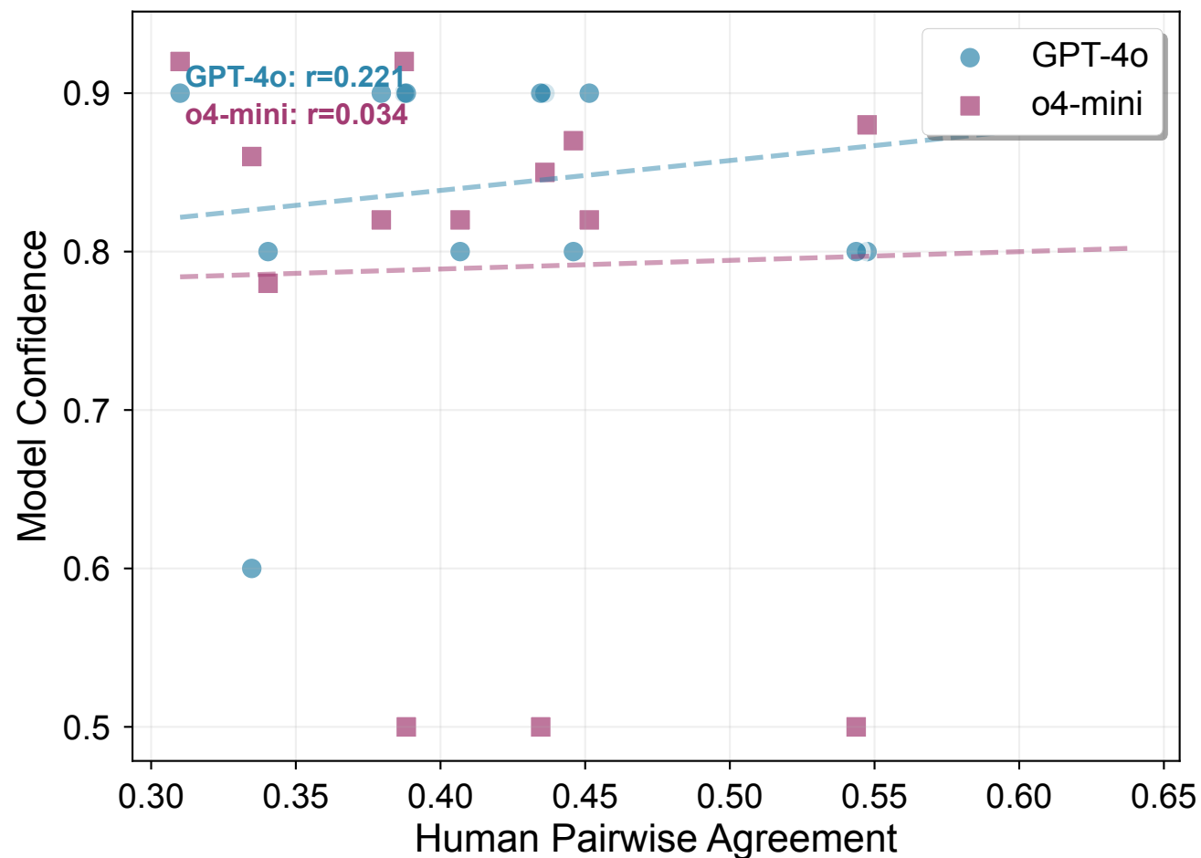
Confidence vs Human Consensus
