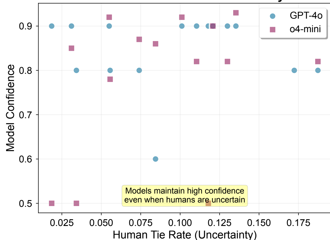
Confidence vs Human Uncertainty
