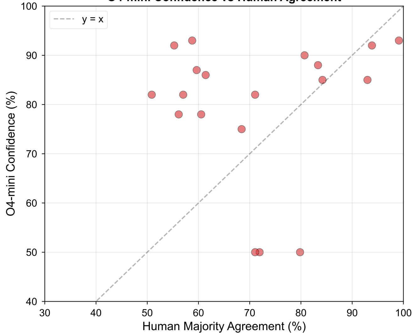
O4-mini Confidence vs Human Agreement
