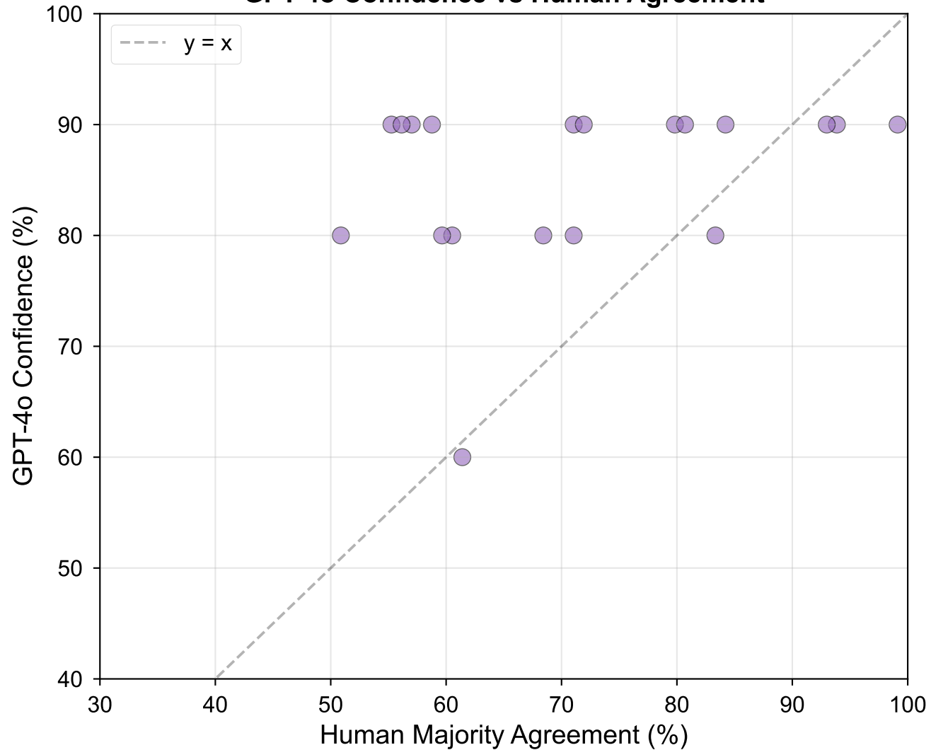
GPT-4o Confidence vs Human Agreement
