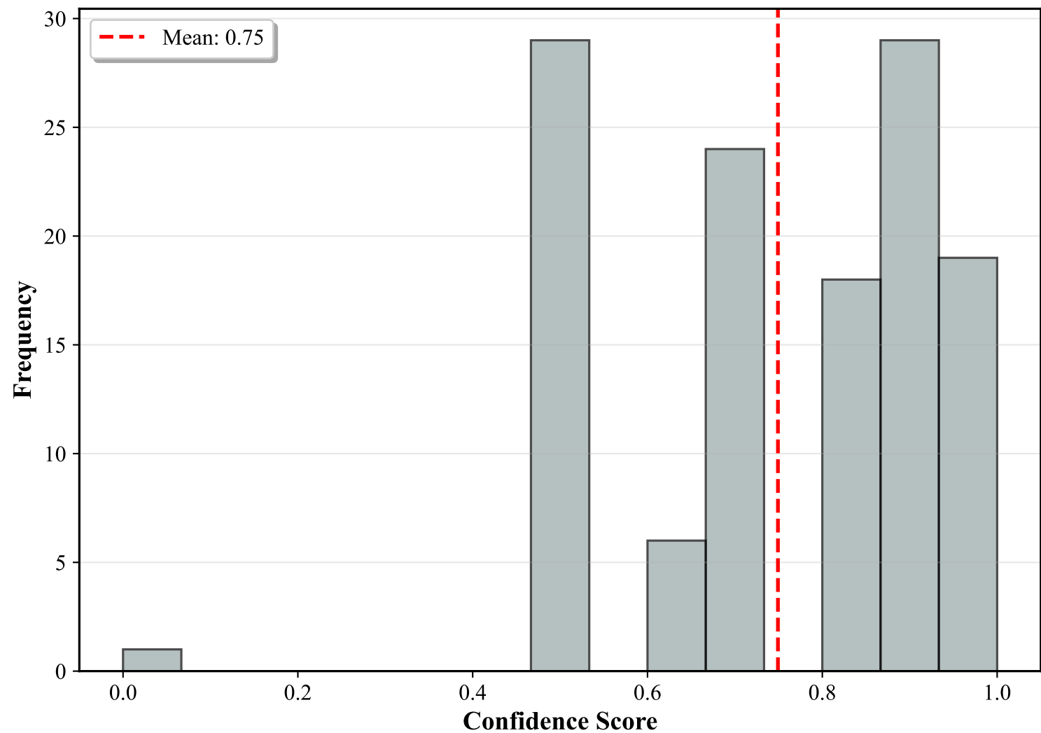
GPT-4o Confidence Distribution
