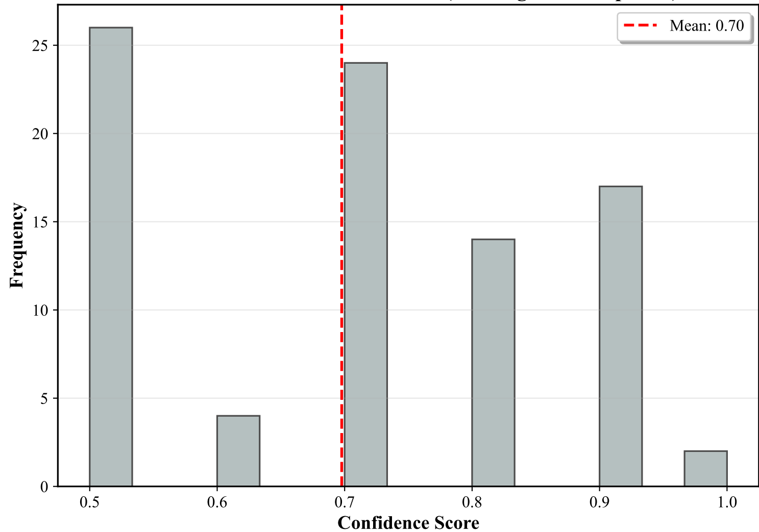
GPT-4o Confidence Distribution (Both Agents Completed)
