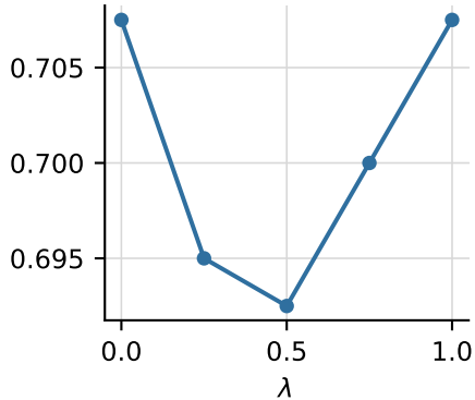
TruthfulQA MC1
