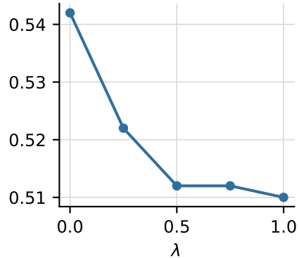
MMLU accuracy
