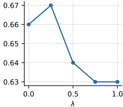
GSM8K accuracy
