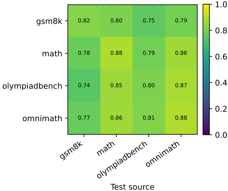
Cross-domain AUROC
