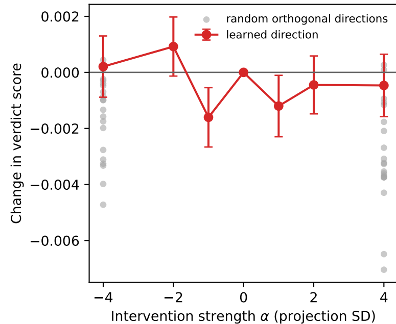
Held-out causal intervention
