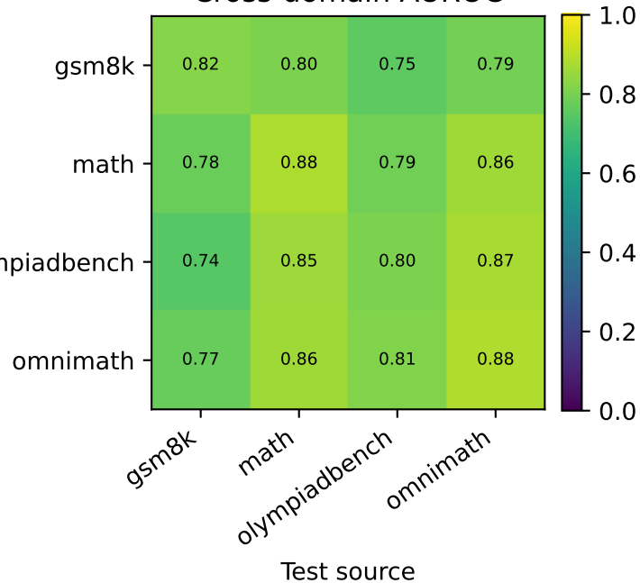
Cross-domain AUROC
