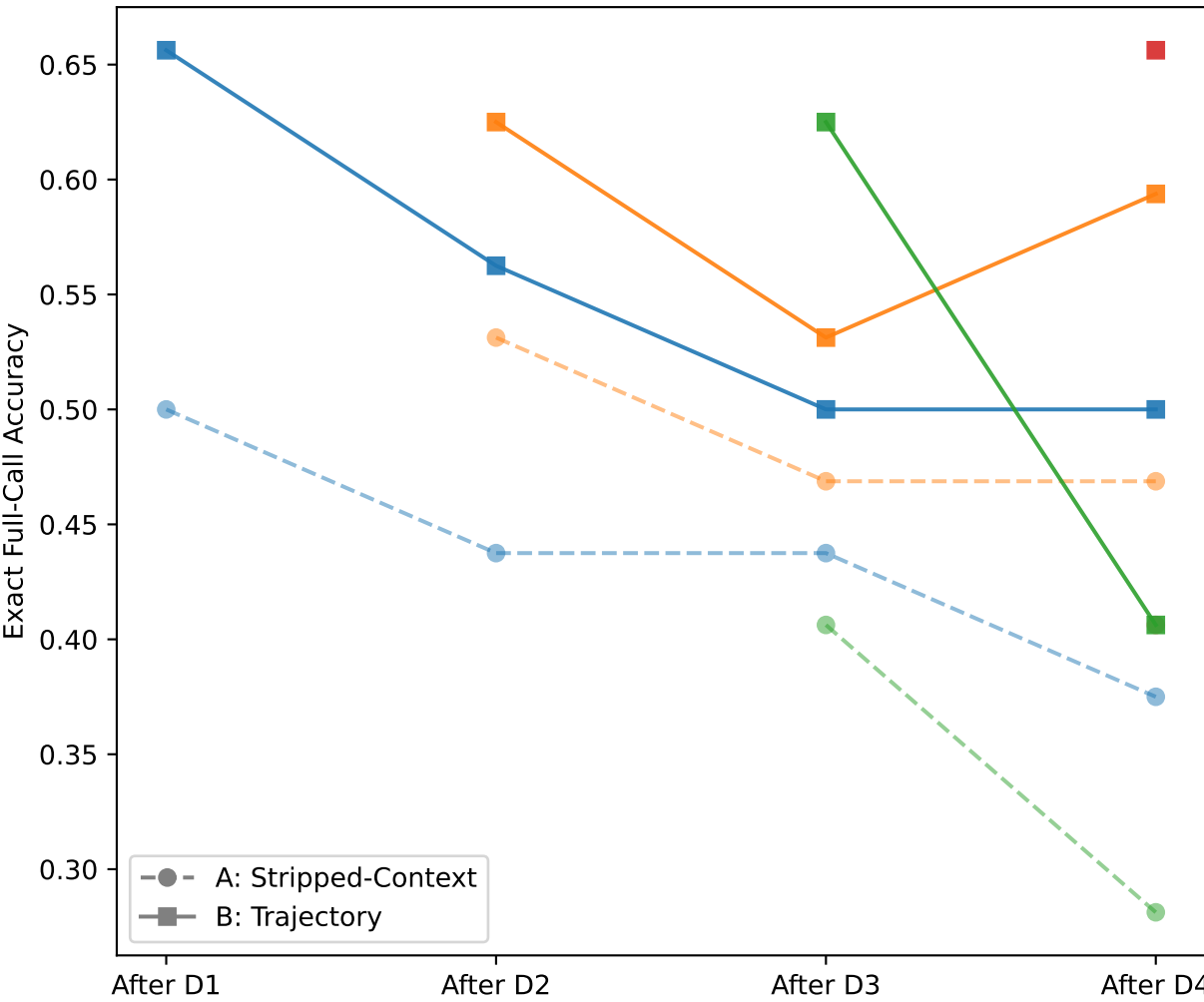
Forgetting Curves
