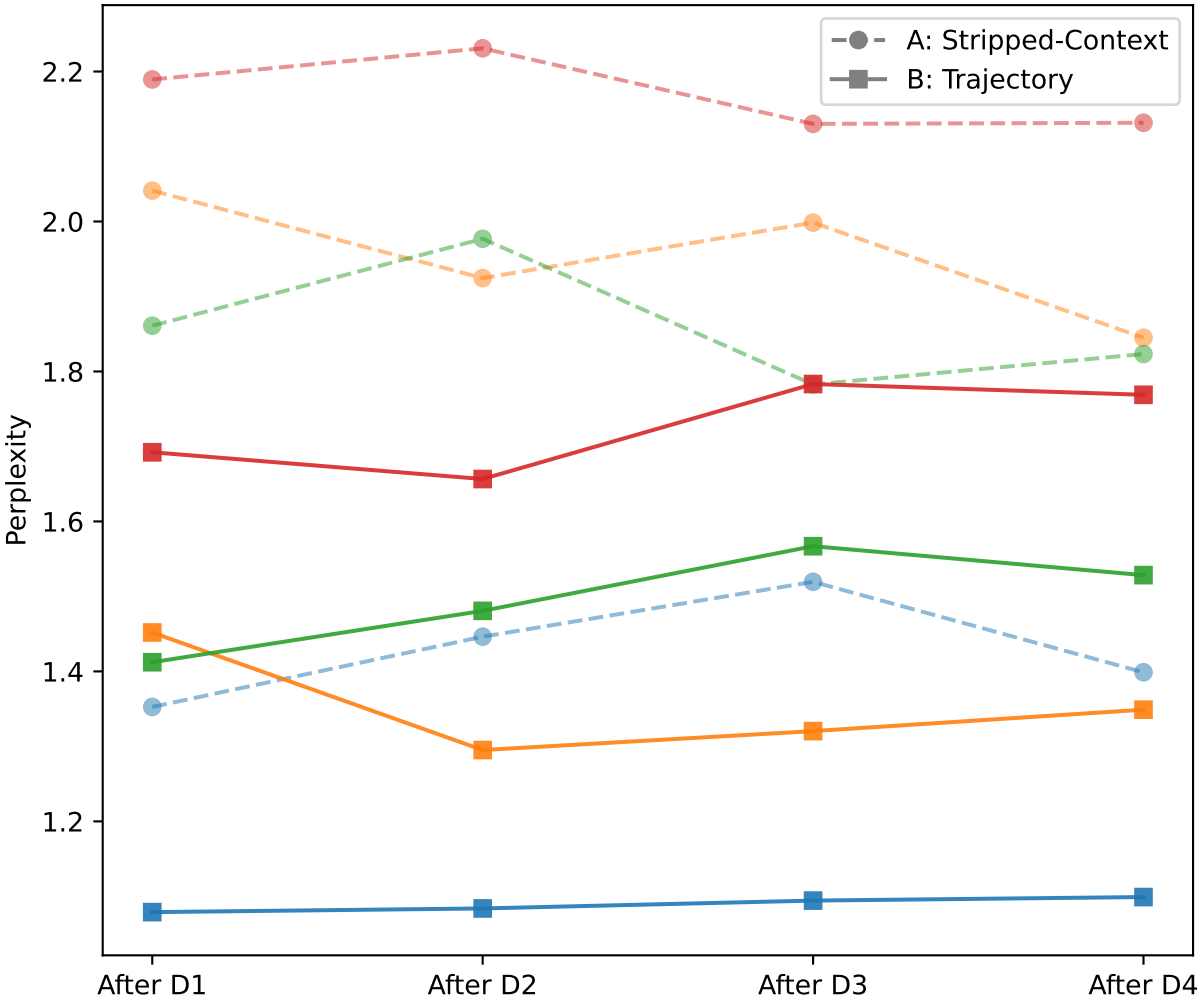
Perplexity Over Time
