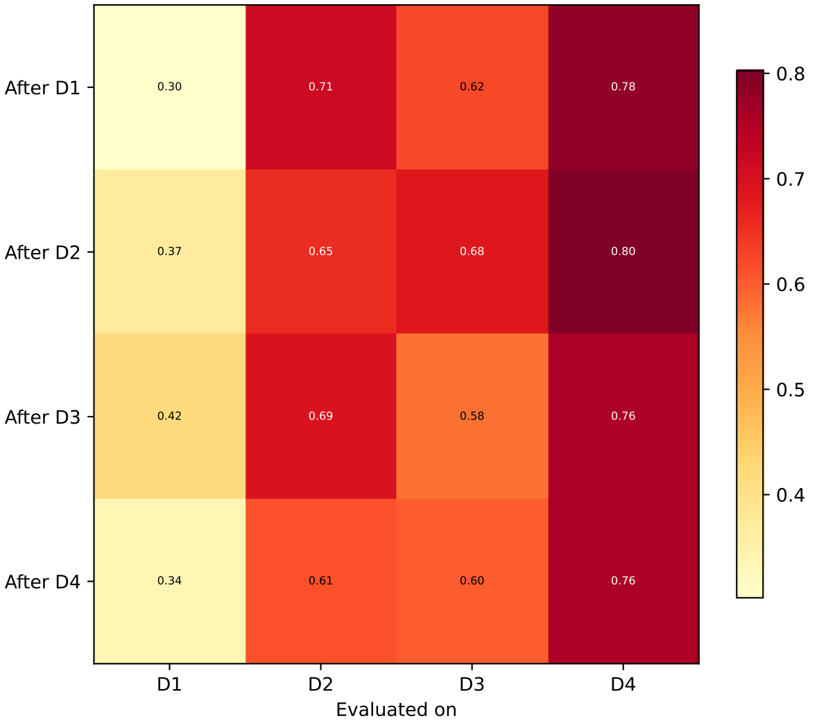
Final Exact Full-Call Accuracy
