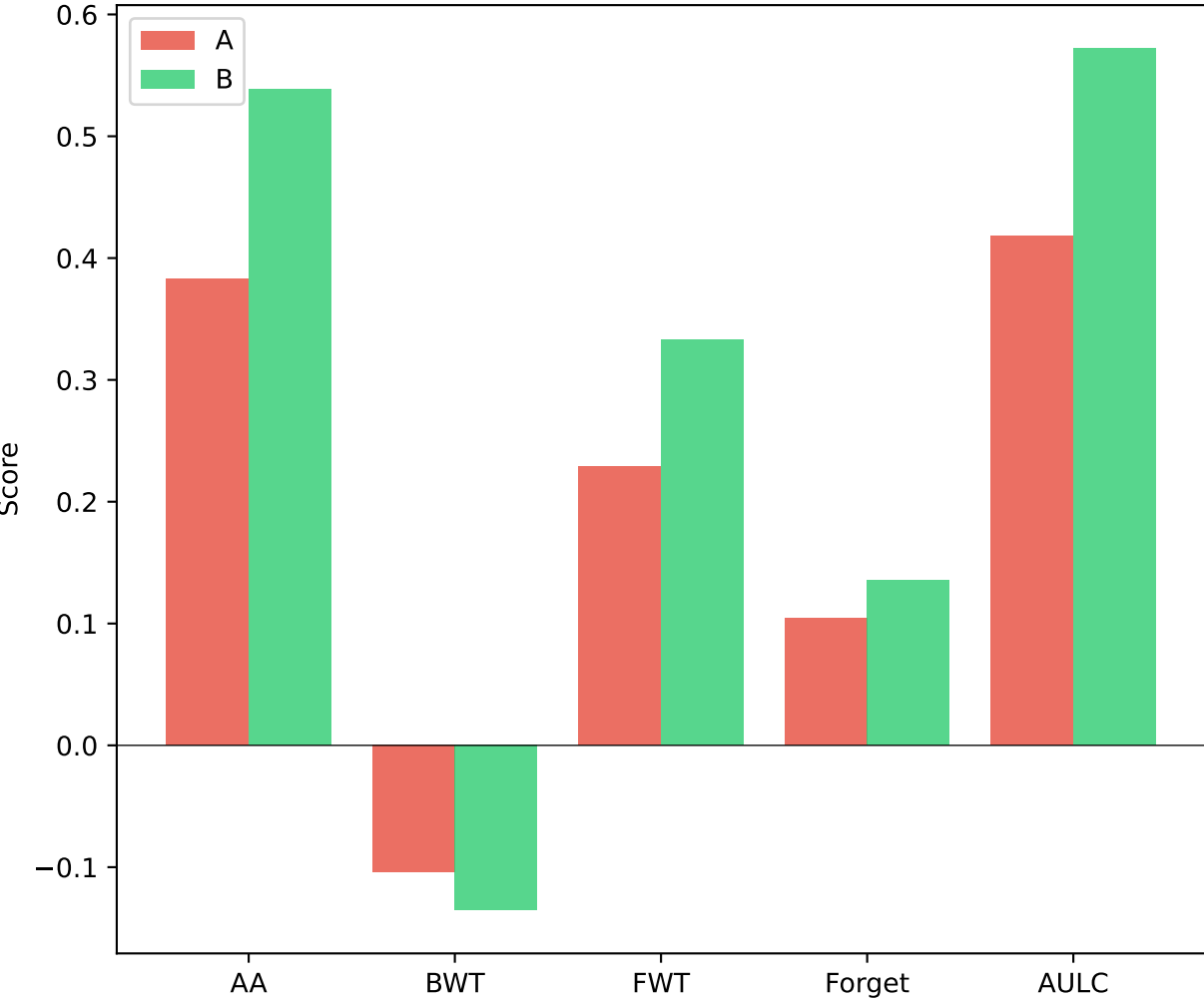
CL Metrics Comparison (Full-Call)
