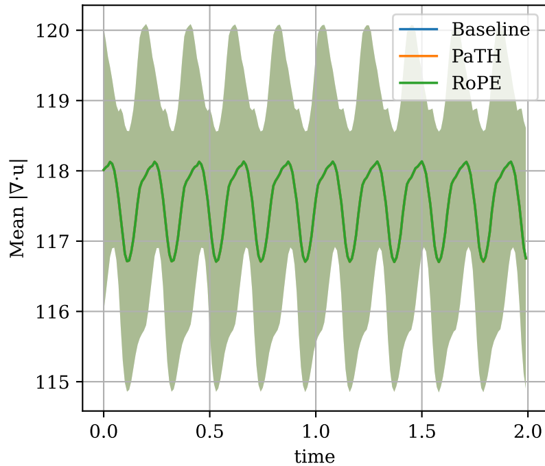
Divergence violation
