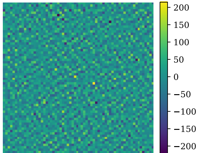
Baseline mean vorticity ( t=1.000 )
