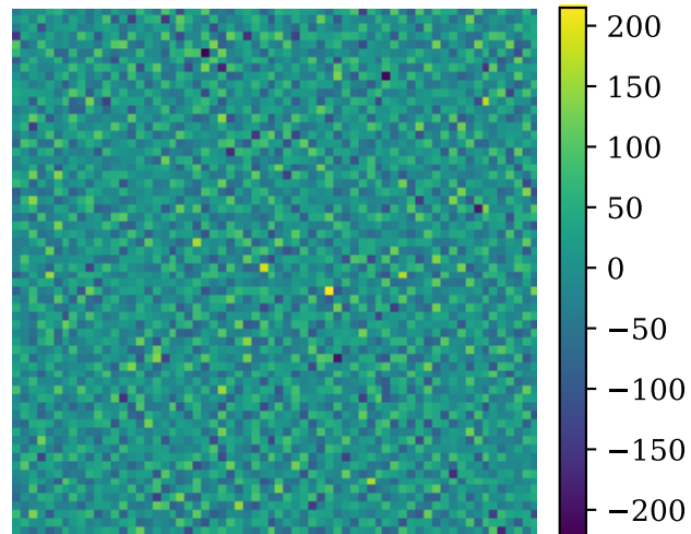
RoPE mean vorticity ( t=1.000 )
