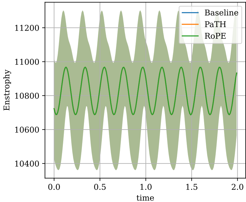
Enstrophy evolution
