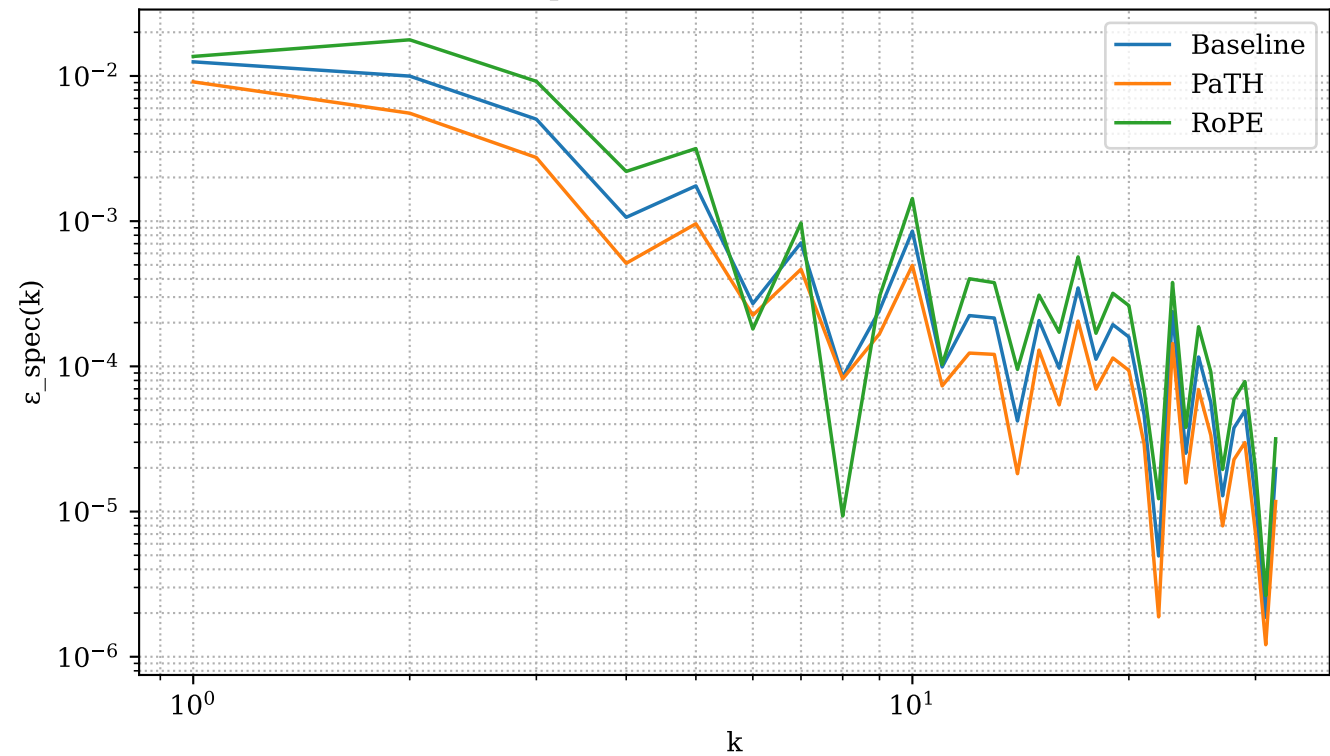
Spectral error at t=1.000
