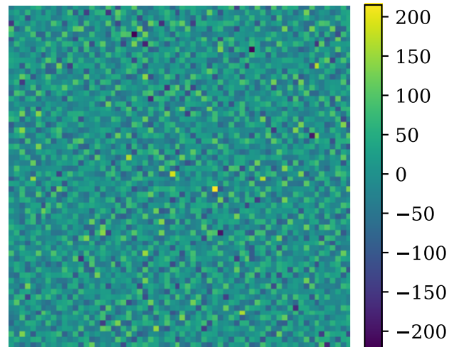
PaTH mean vorticity ( t=1.000 )
