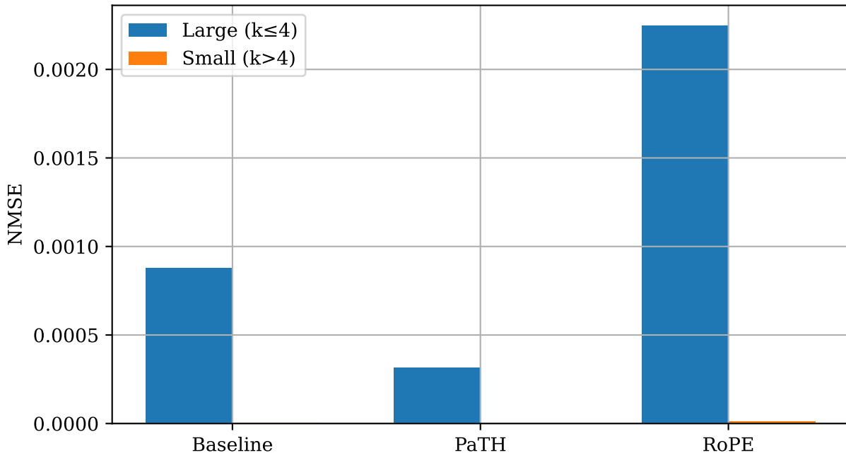
Scale-dependent NMSE (mid time)
