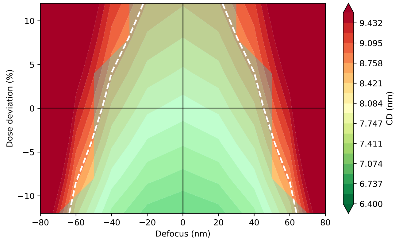
(B) High-NA (NA=0.55, \epsilon=0.13 ) In-spec: 33/63 (52%)
