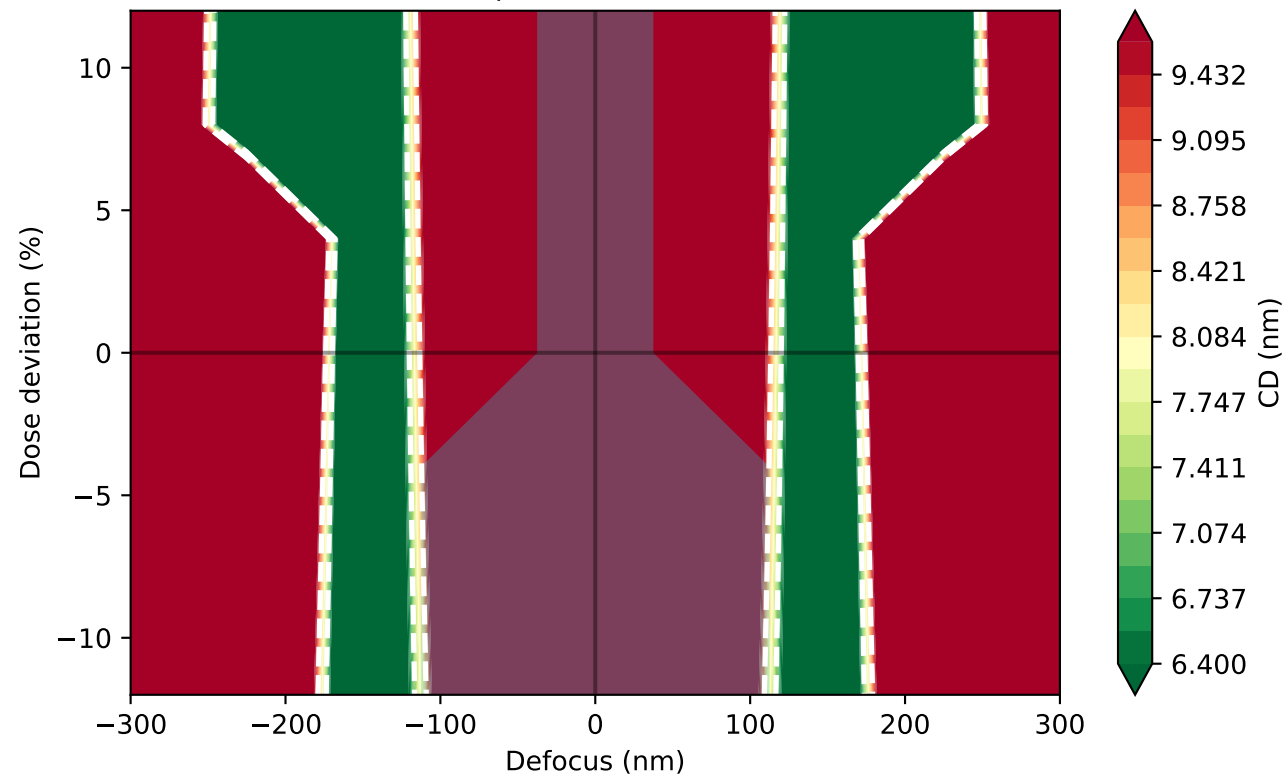
(A) Conventional (NA=0.33, no obsc.) In-spec: 13/63 (21%)
