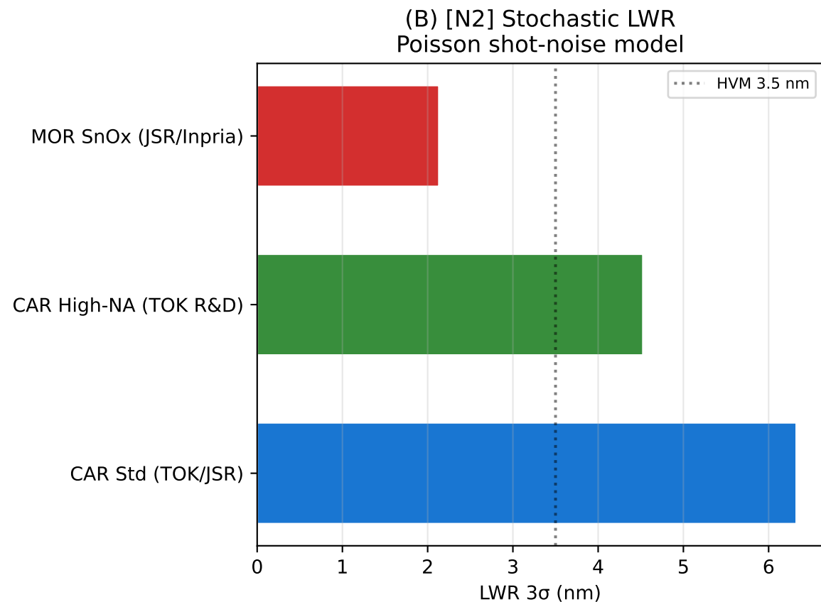
Figure 6: MC CDE + [N2] Stochastic LWR + [N3] RLS Triangle
