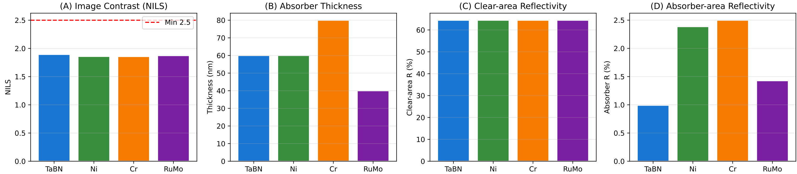
Figure S2: Absorber Comparison — PTB-2022 n/k + Correct Stack Geometry (BUGFIX-2) [N5]
