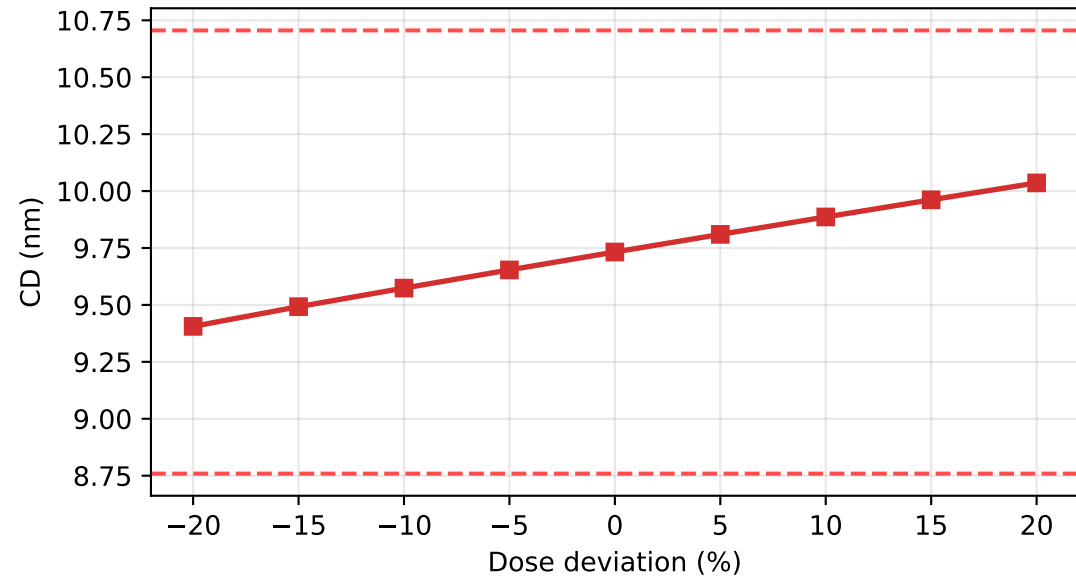
(B) CD vs Dose (High-NA, dipole) EL_sim=40.0% Benchmark=40.0%
