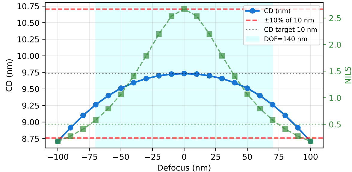
(A) CD & NILS vs Defocus (High-NA, dipole) DOF_sim=140 nm Benchmark=140 nm
