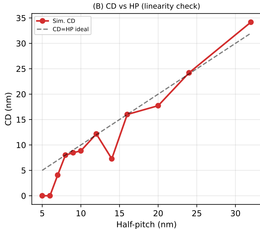
Figure S4: Through-Pitch Analysis
