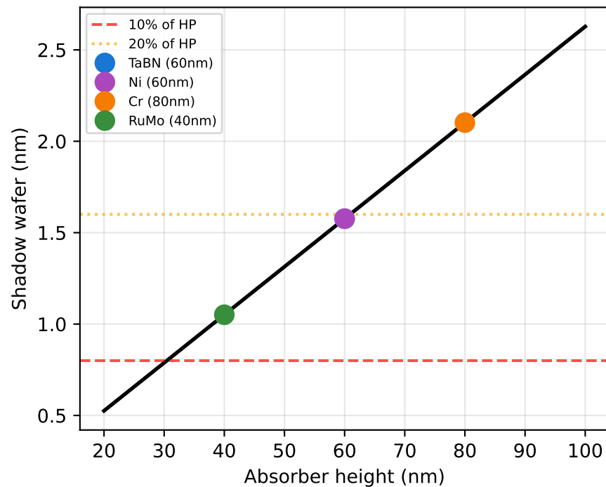
(B) Shadow vs Absorber Height
