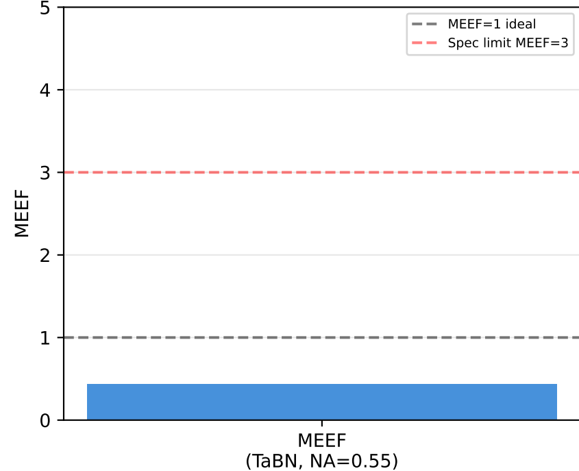
(C) MEEF = 0.44 ( \pm 1 nm mask CD, Mx=4)
