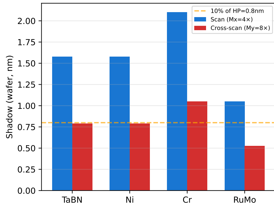
(A) 3D Mask Shadow Bias ( \theta=6^\circ )
