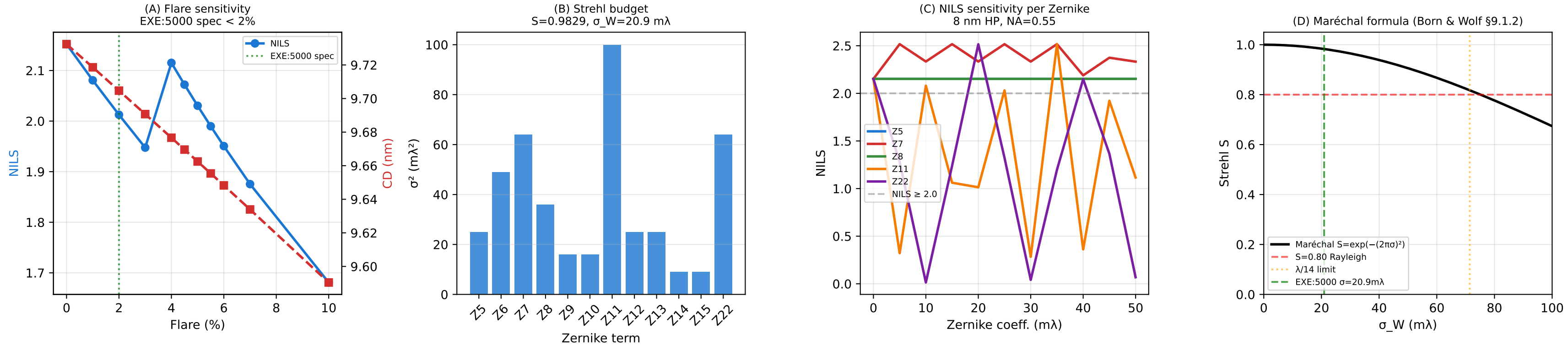
Figure S6: Flare Sensitivity + Strehl Budget
