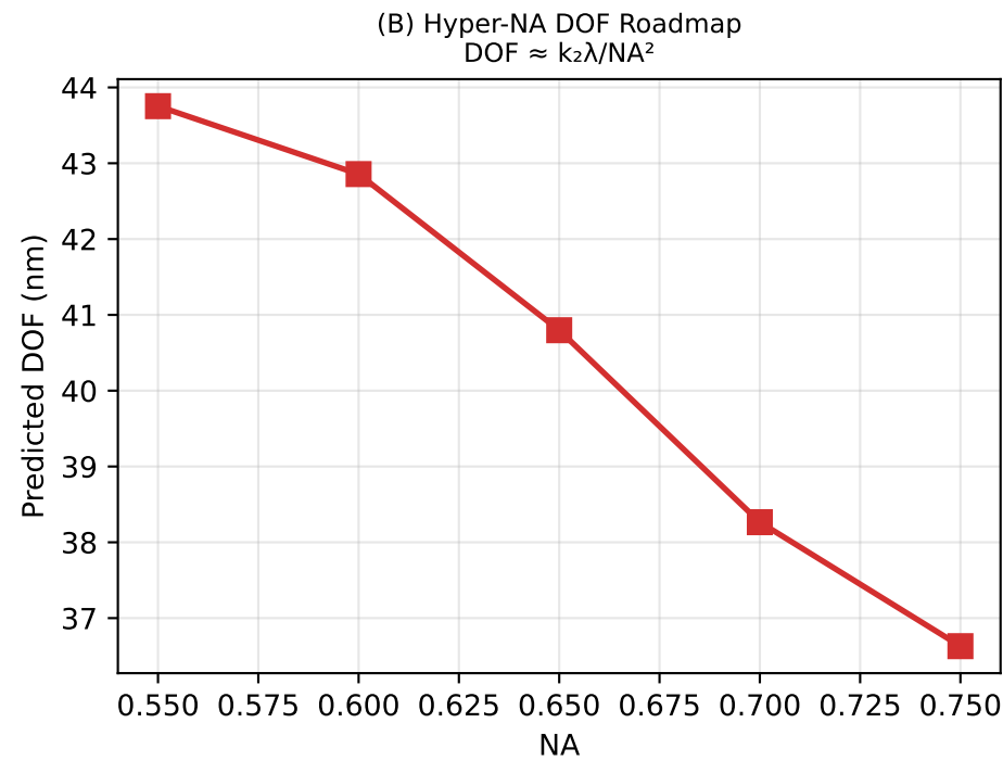
Figure S9: Hyper-NA Roadmap + Apodization
