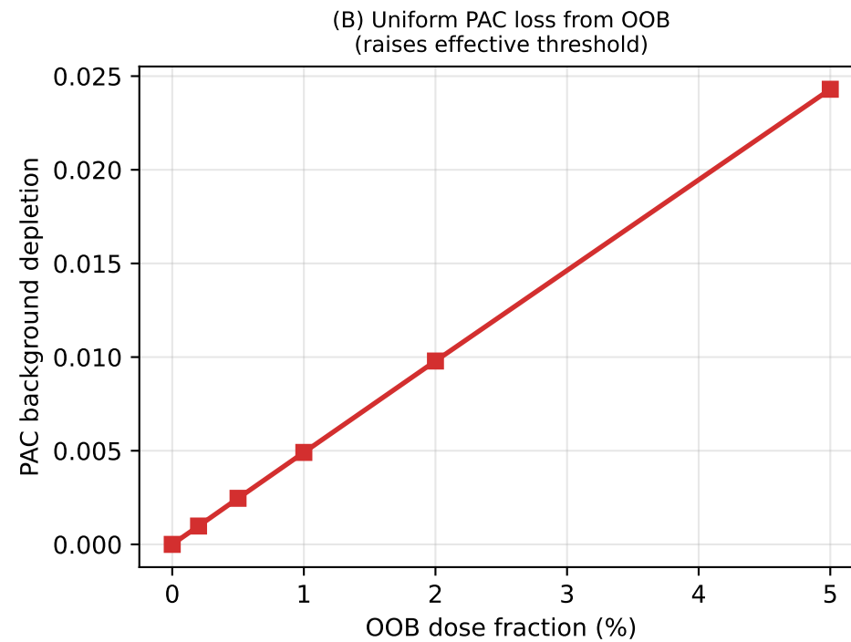
Figure S10: OOB + Plasma Charging + Mack-4 + 3D EM
