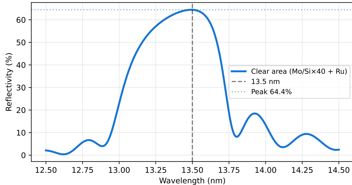
(A) Clear-Area Reflectivity (no absorber) PTB-2022 Mo/Ru constants
