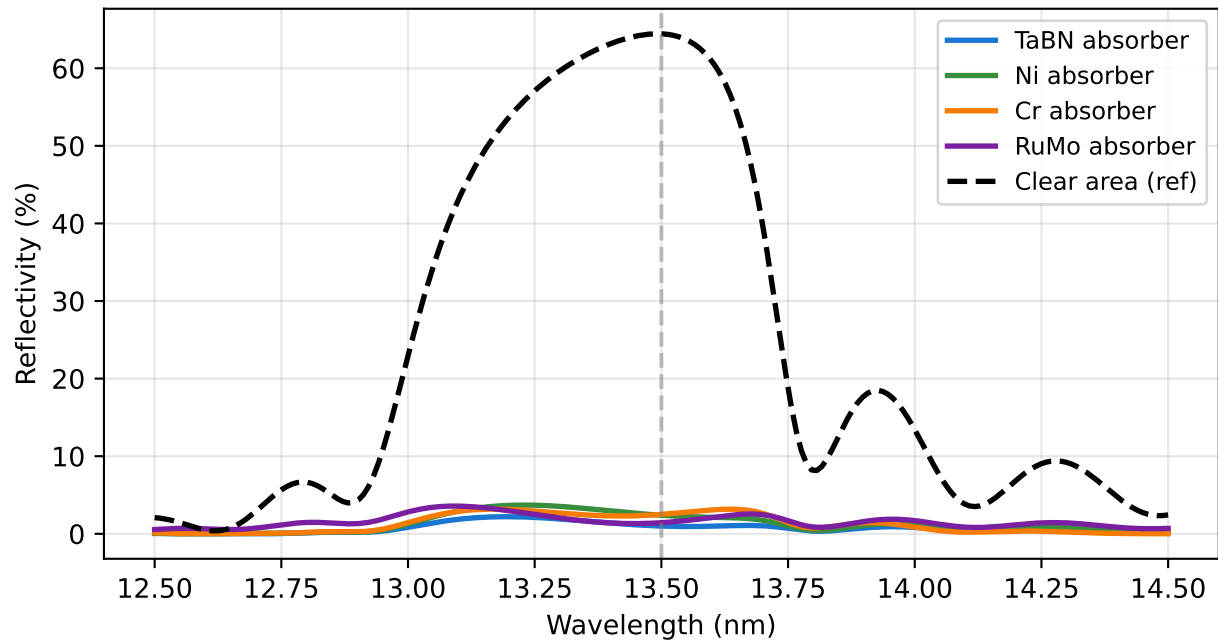
(B) Absorber-Area R vs Clear-Area R Mask contrast visualisation
