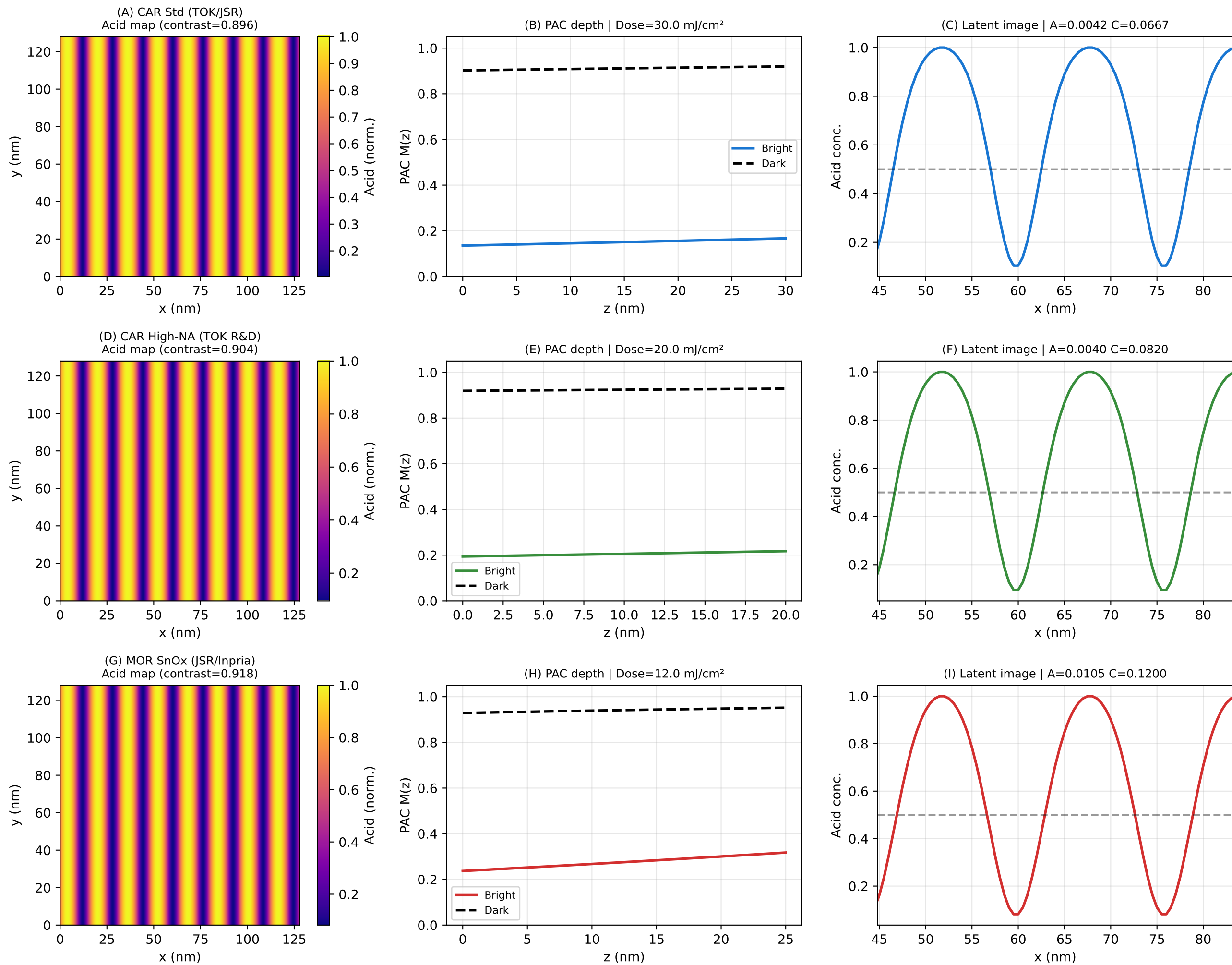
Figure 4: Updated Dill Resist Model — 3 Classes (CAR std, CAR HiNA, MOR SnOx) [N5]
