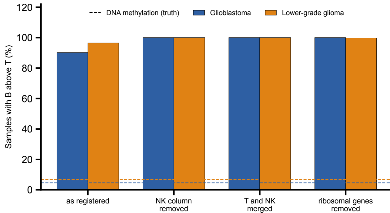
A B above T, by reference variant (SVR)
