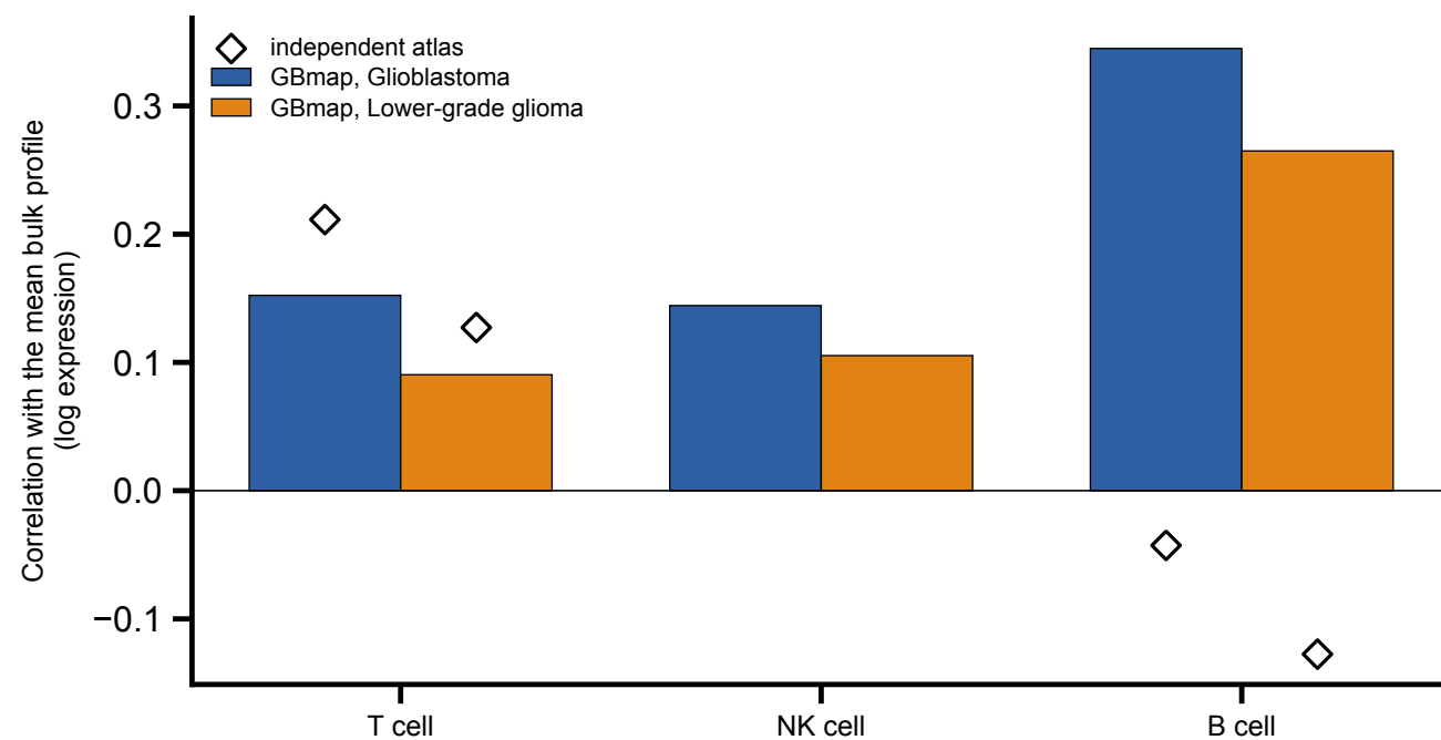
C Similarity of each lymphoid profile to bulk tumour
