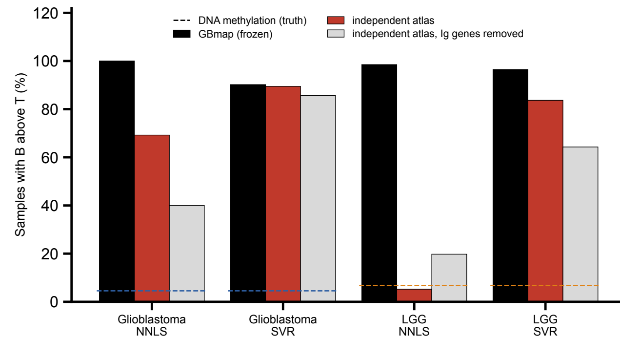
D B above T: GBmap versus an independent atlas
