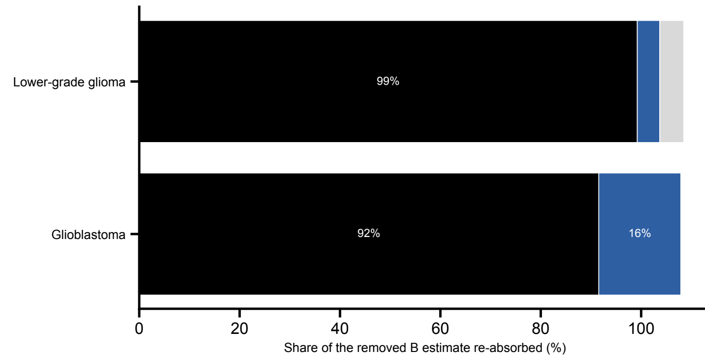
B Where B's estimate goes when B is removed (SVR; under NNLS it goes to T instead)
