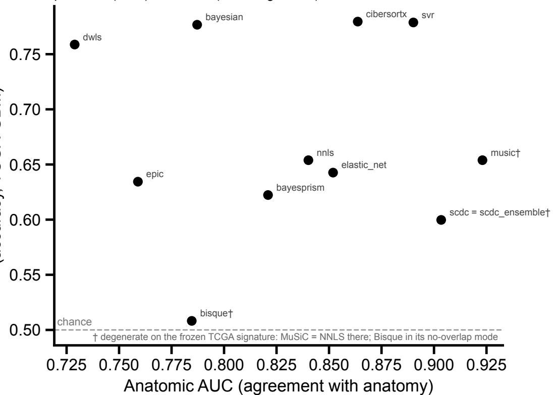
B Neither anatomy score tracks accuracy \rho = -0.06 (AUC) vs +0.081 (ACS, registered); n = 12
