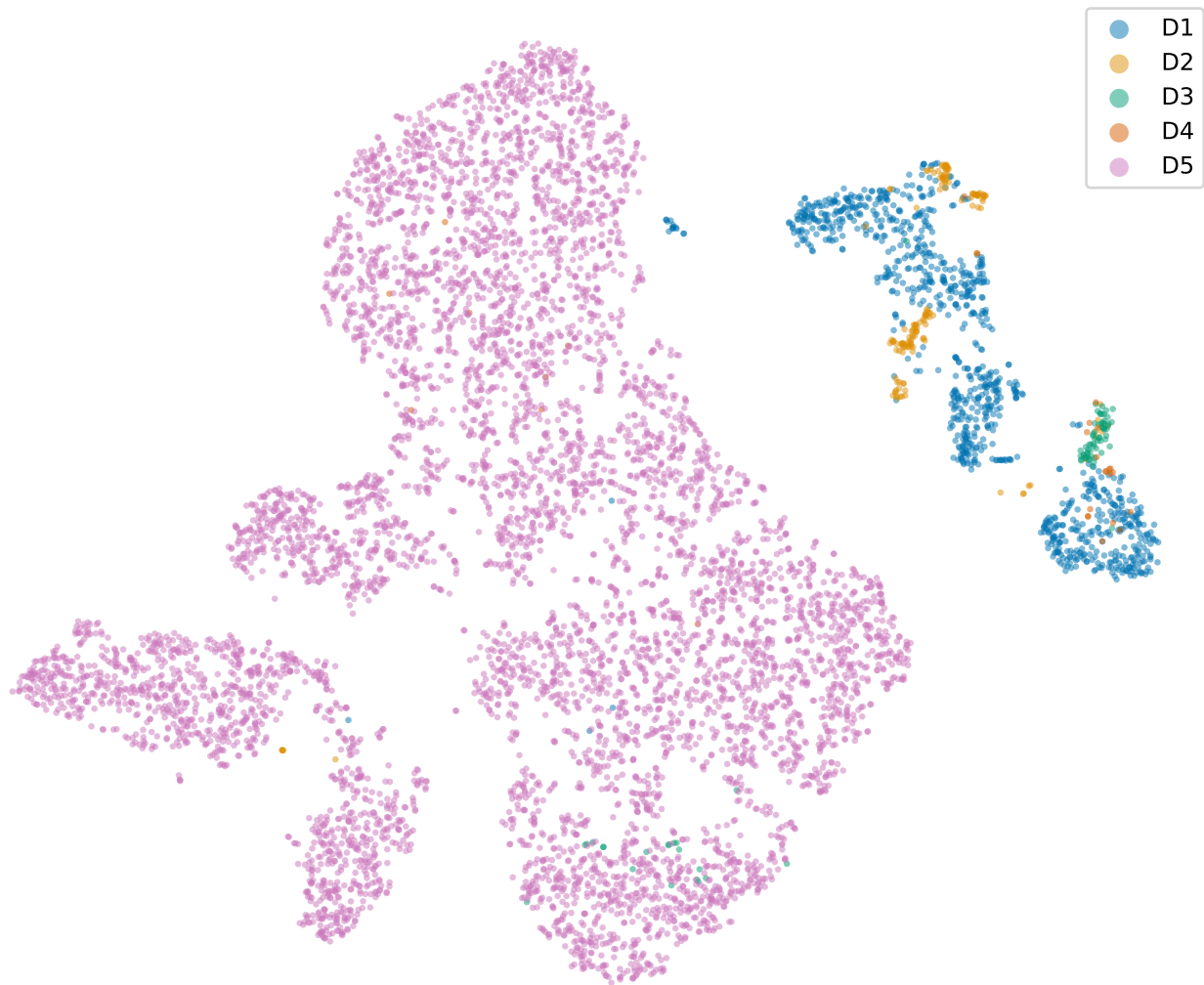
t-SNE of B1 embeddings — coloured by domain
