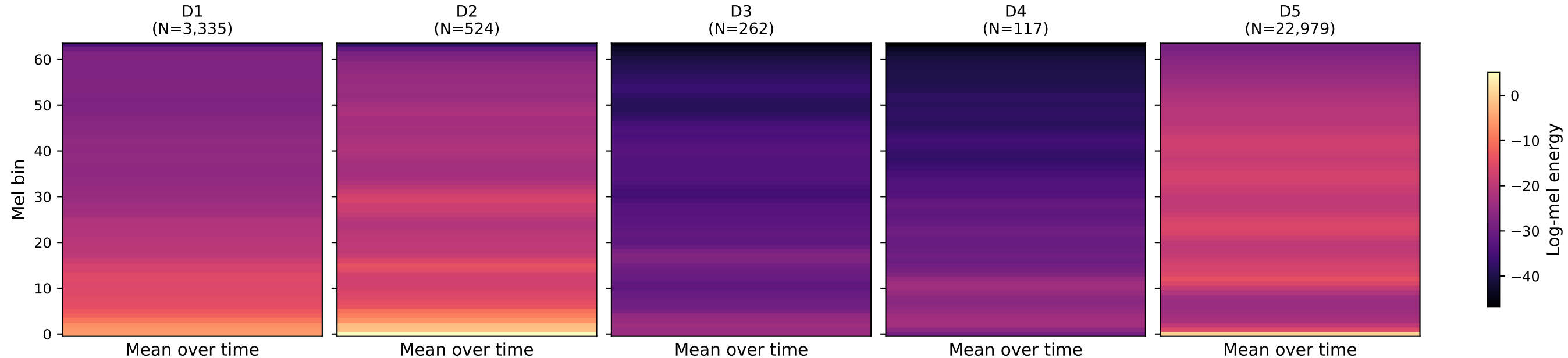
Mean log-mel spectrum per recording domain (test set)
