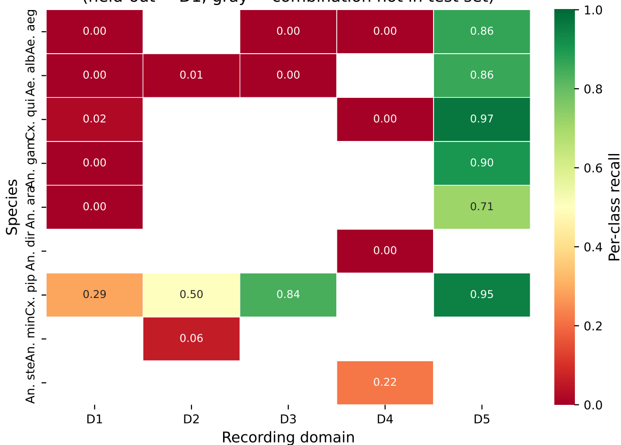
Per-species recall by domain — B1 baseline LODO-D1 test (held-out = D1; gray = combination not in test set)
