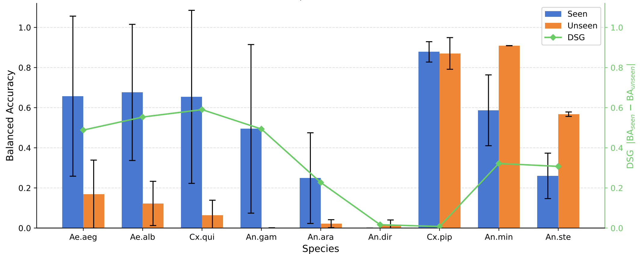
Per-Species Evaluation: balanced_dann_dicl_proj128_τ=0.2 (LODO D1-D4, best checkpoint, error bars = std across folds)
