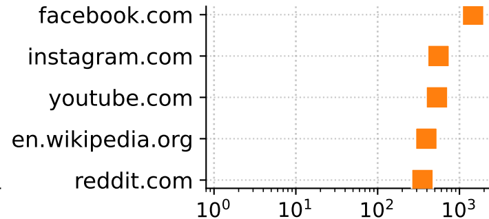
Grok-4.3
