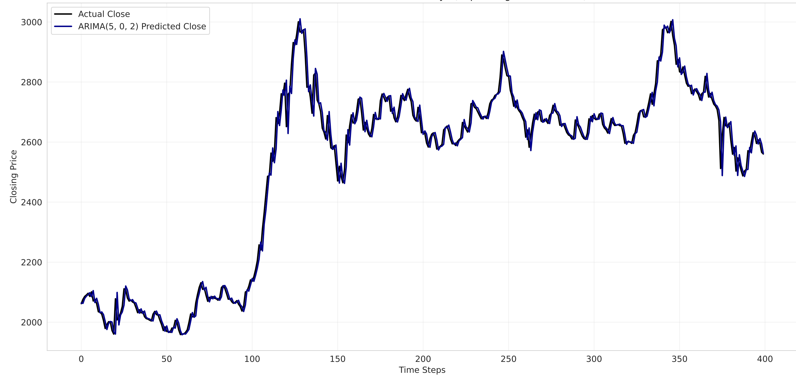
NEPSE Index Forecast - Last 400 Days (Expanding, Tuned ARIMA)
