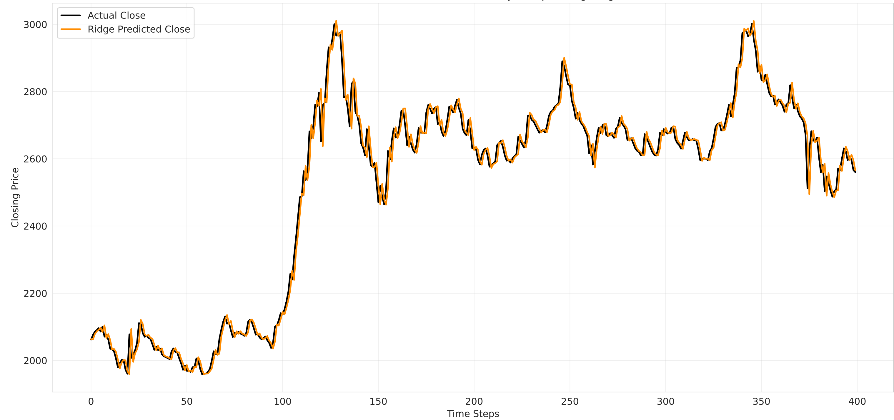
NEPSE Index Forecast - Last 400 Days (Expanding, Lag=10)
