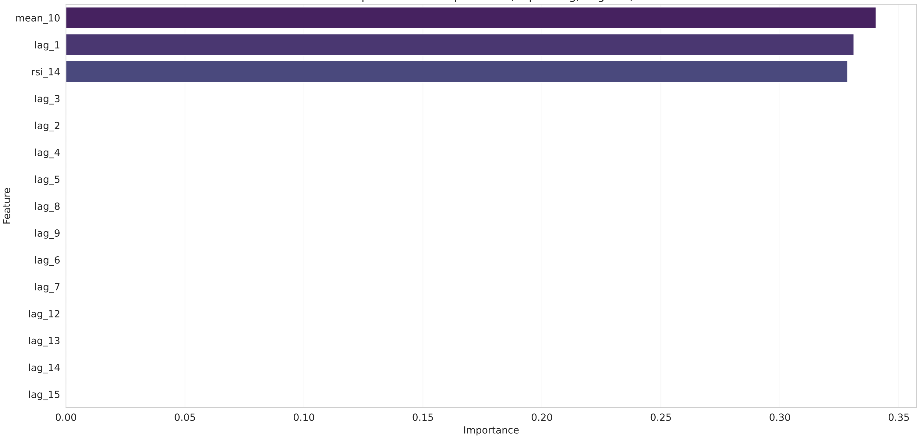
Top 15 Feature Importance (Expanding, Lag=30)
