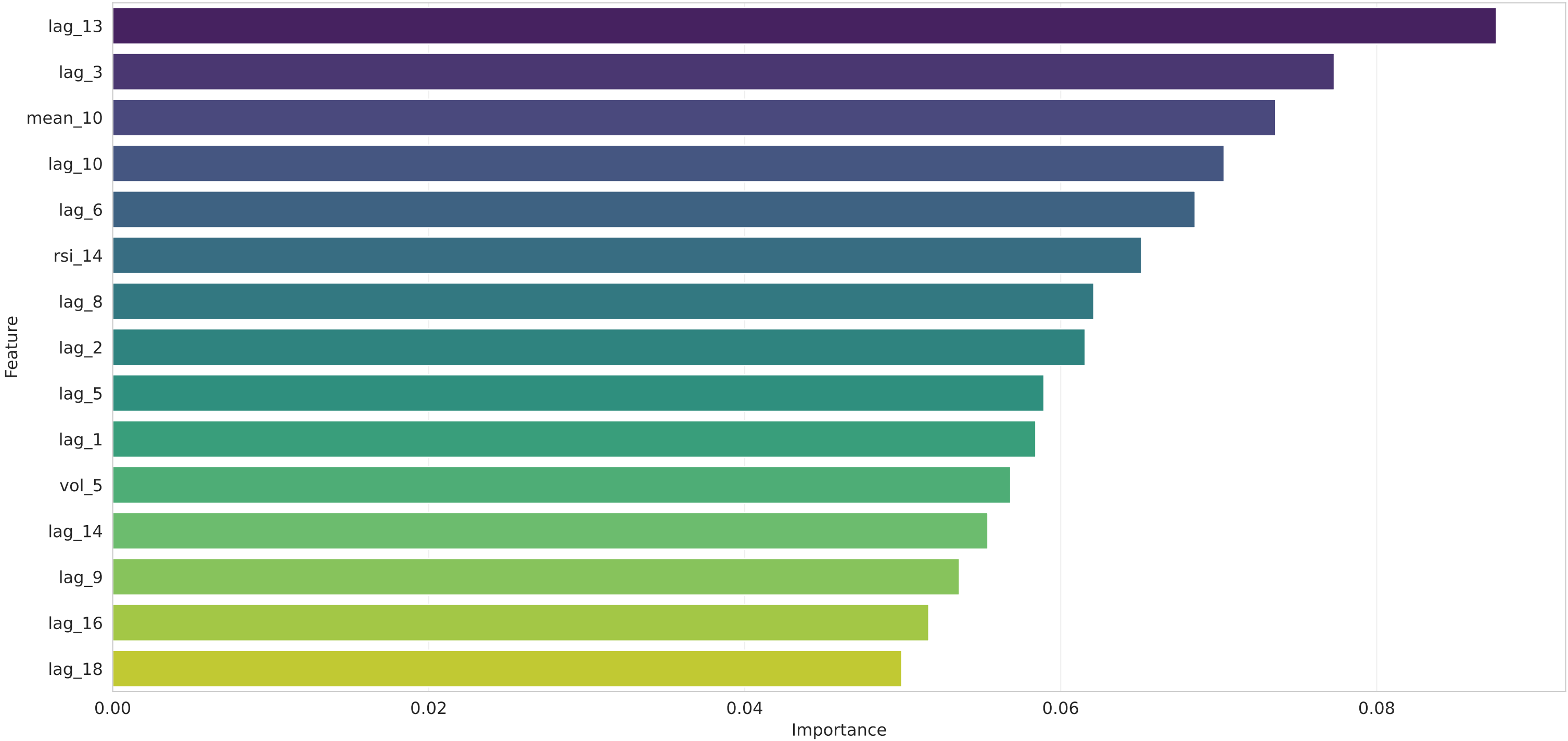
Top 15 Feature Importance (Rolling, Lag=20)
