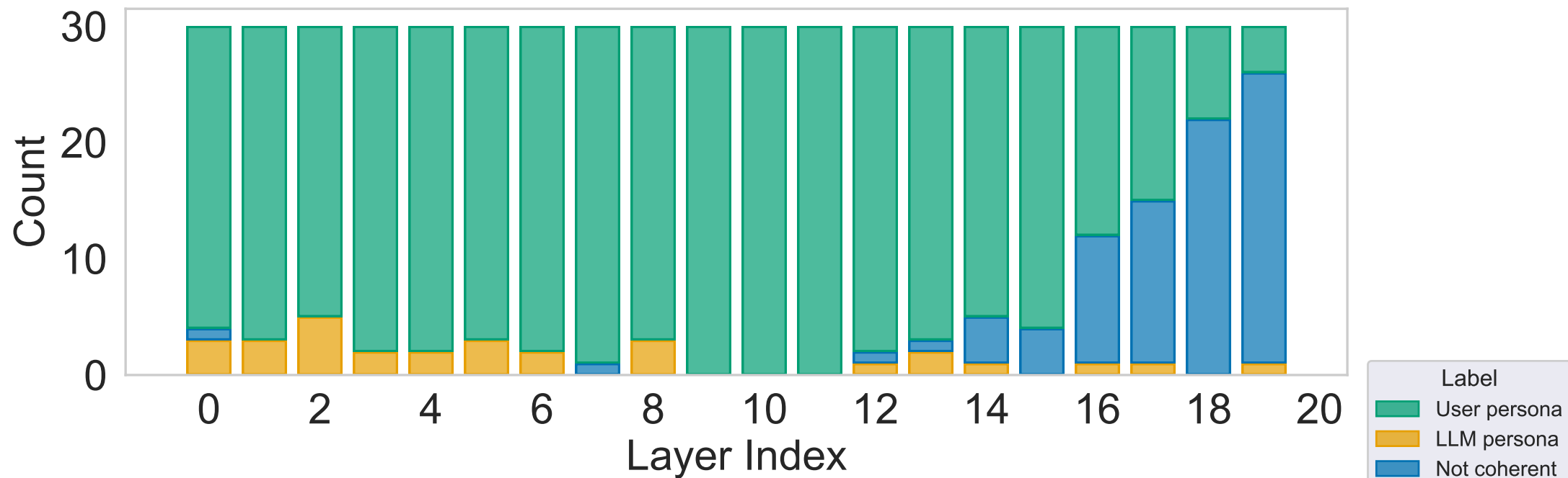
Steer towards 'I'
